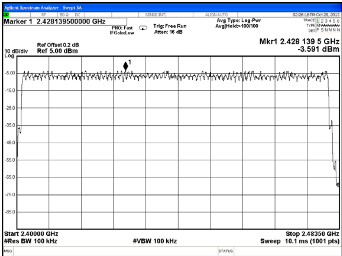
Figure 1: 8-DPSK
