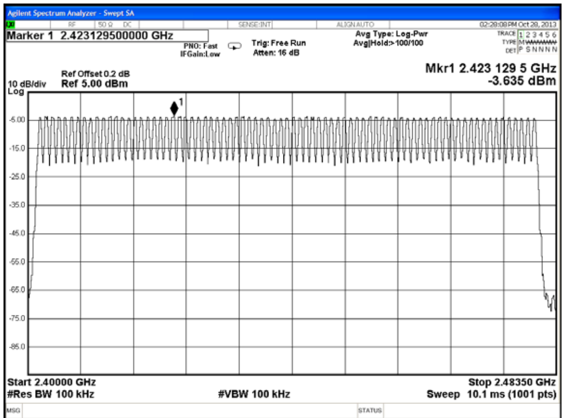
Figure 2: GFSK
