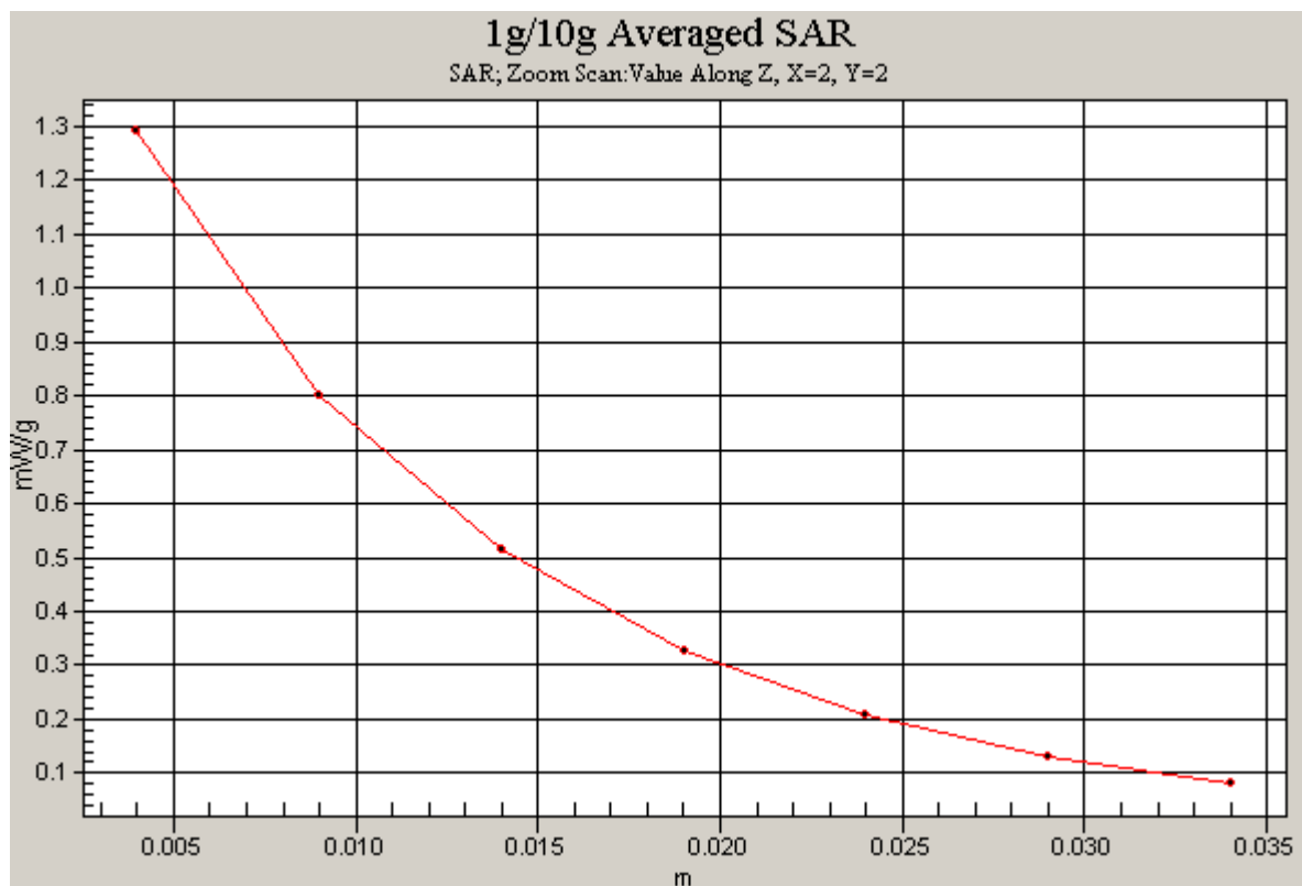
Figure 38 Body, Towards Ground, GSM 1900 GPRS (4 timeslots uplink) SIM1 Channel 512
