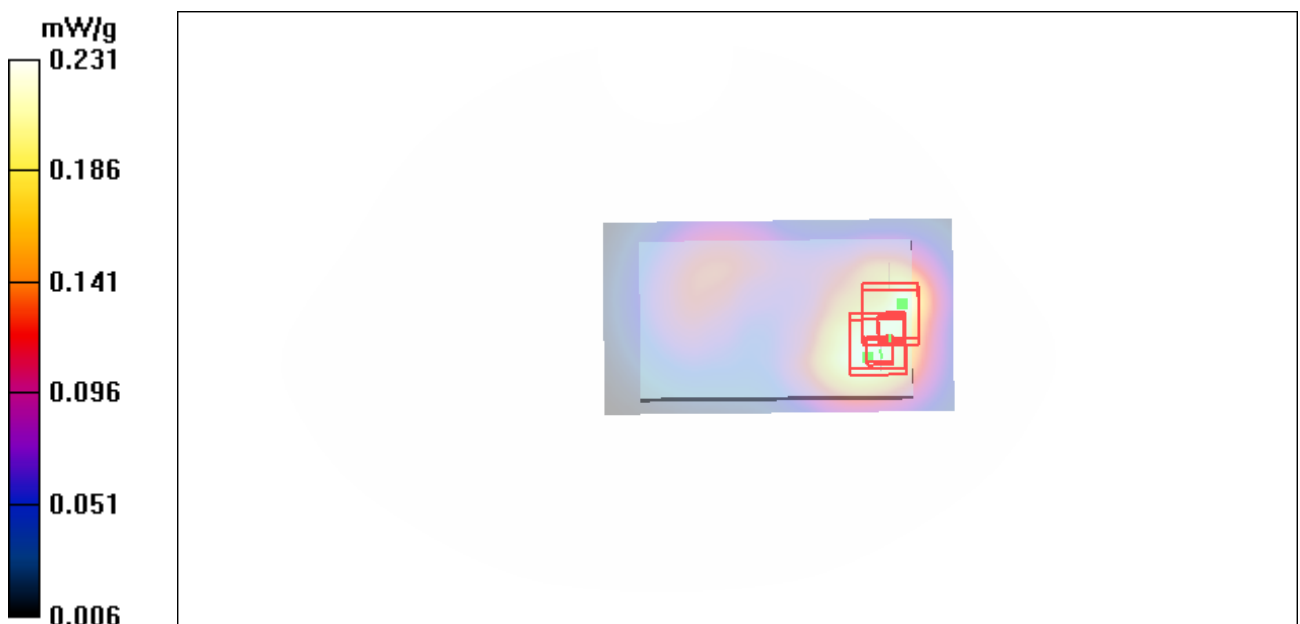
Figure 32 Body, Towards Ground, GSM 1900 SIM1 Channel 810
