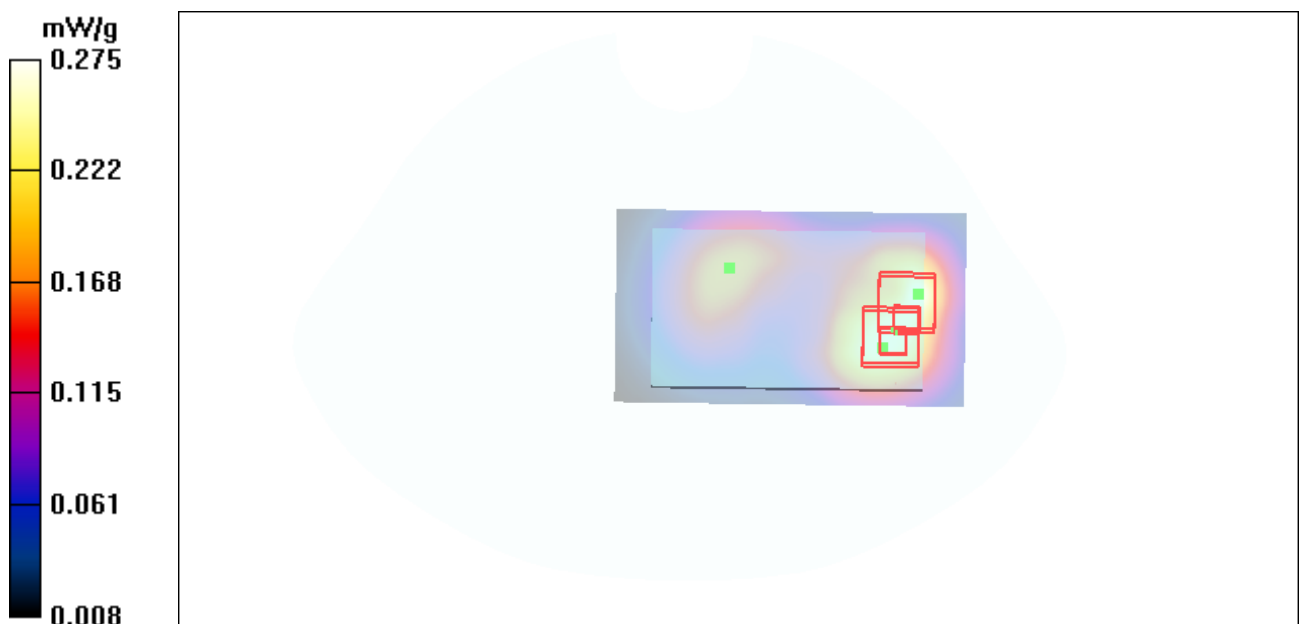
Figure 33 Body, Towards Ground, GSM 1900 SIM1 Channel 661
