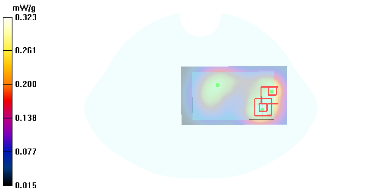
Figure 36 Body, Towards Ground, GSM 1900 SIM2 Channel 512
