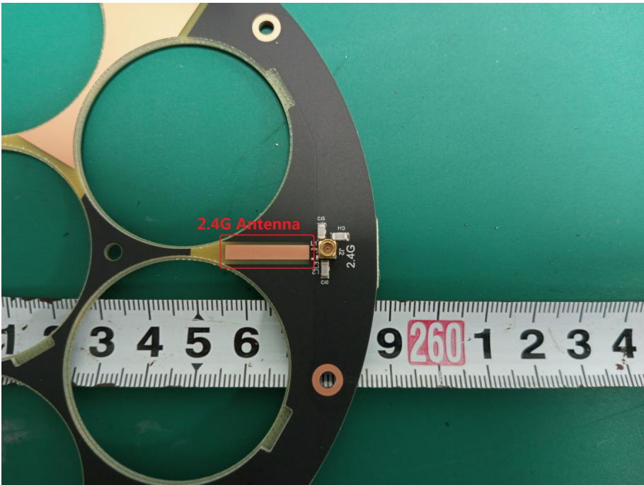
UHF Antenna
