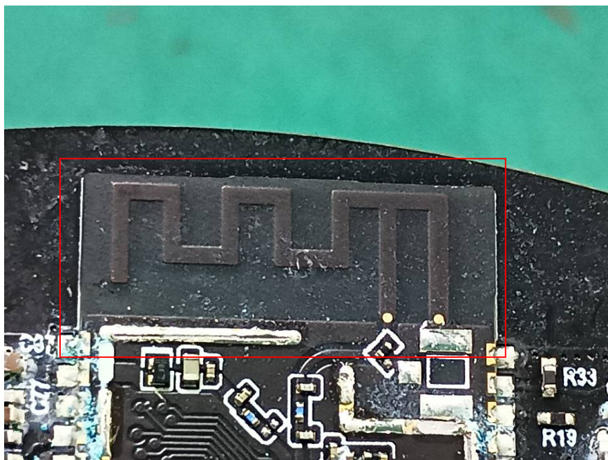
BT/Wi-Fi ANT
