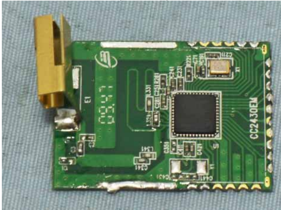
Figure 13 PCB of the EUT-Front View (RF Module)
