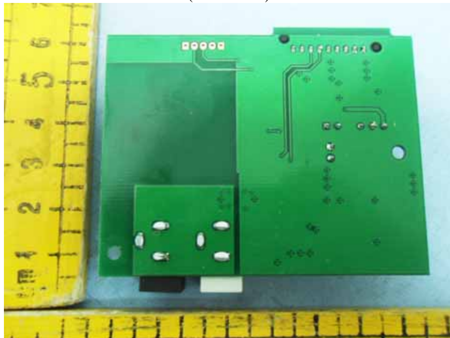
Figure 12 PCB of the EUT-Back View (RF Module)
