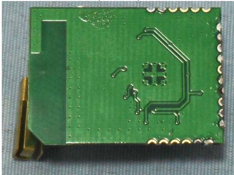
Figure 14 PCB of the EUT-Back View (RF Module)
