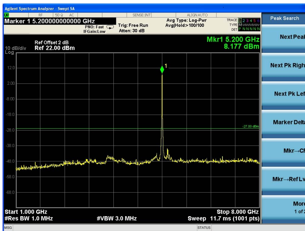
(Plot 4.9.1 B4: Channel 40: 5200MHz @ 802.11a)
