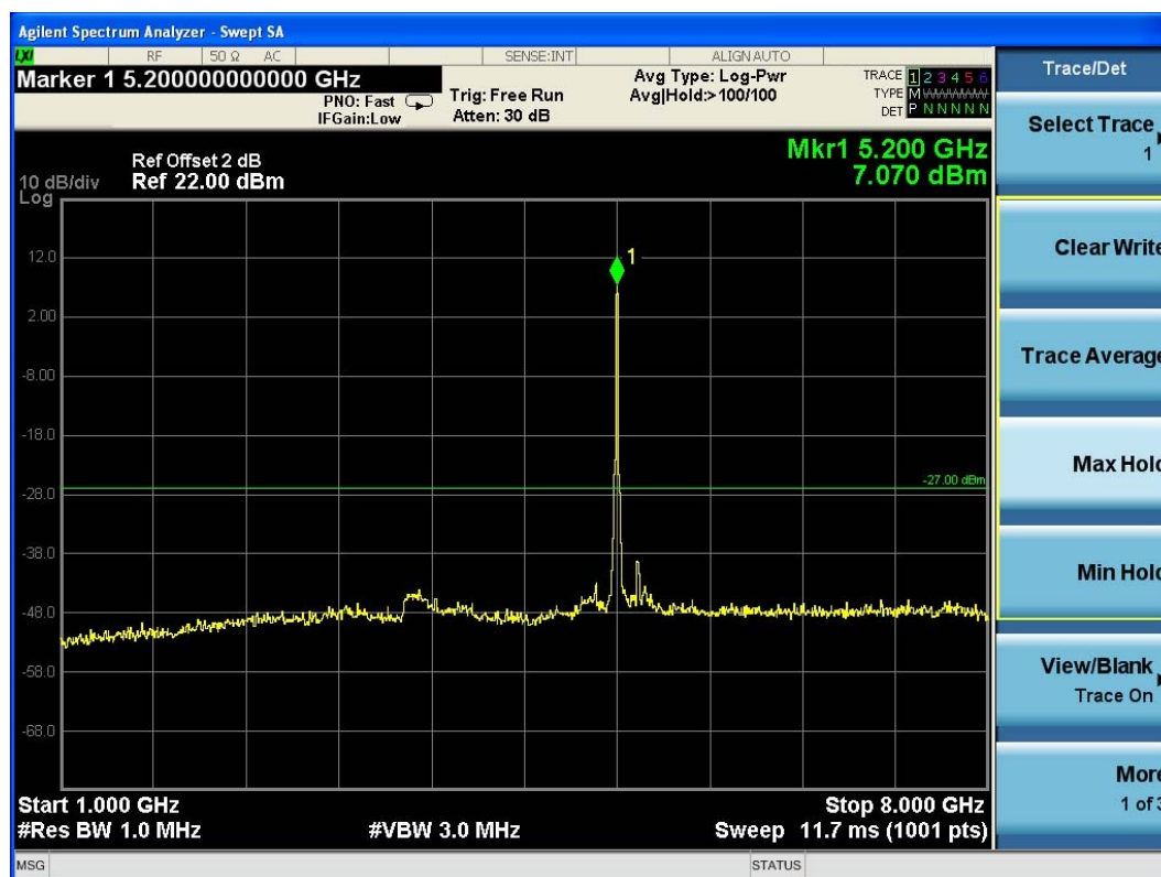
(Plot 4.9.2 B4: Channel 40: 5200MHz @ 802.11n HT20)
