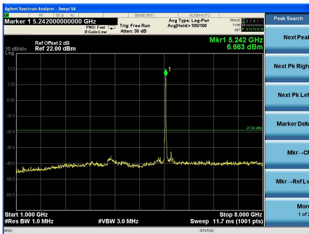
(Plot 4.9.2 C4: Channel 48: 5240MHz @ 802.11n HT20)
