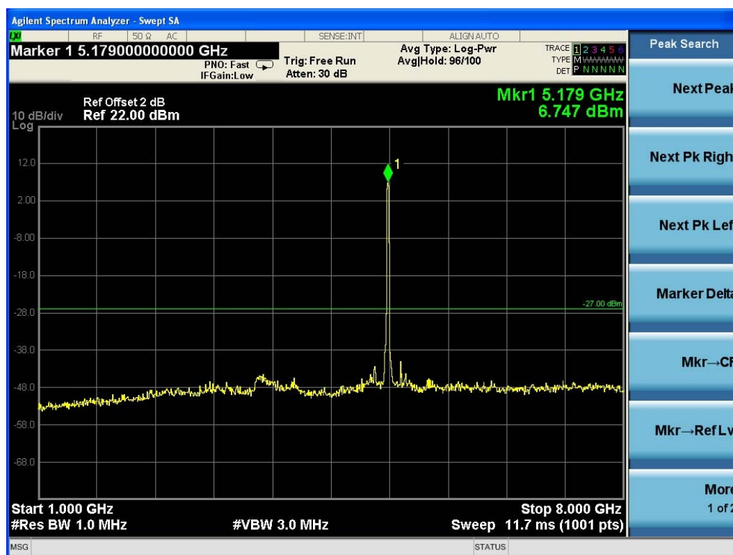
(Plot 4.9.2 A4: Channel 36: 5180MHz @ 802.11n HT20)
