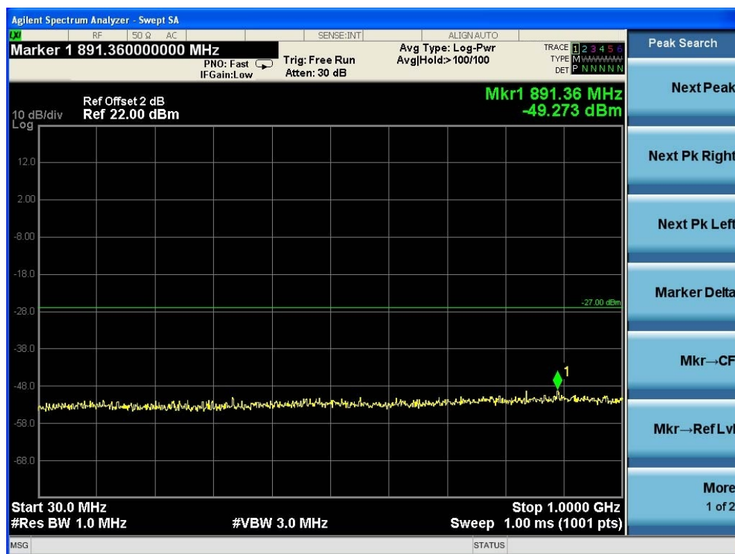
(Plot 4.9.2 A3: Channel 36: 5180MHz @ 802.11n HT20)
