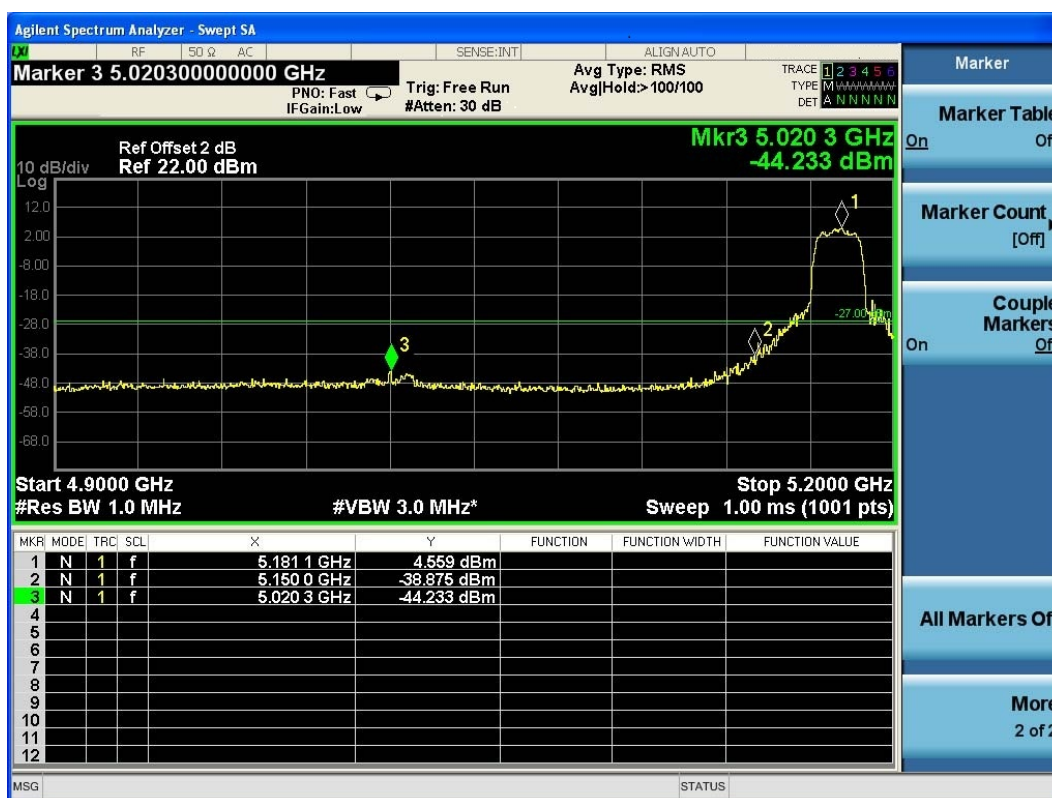
(Plot 4.9.1 A1: Channel 36: 5180MHz @ 802.11a)
