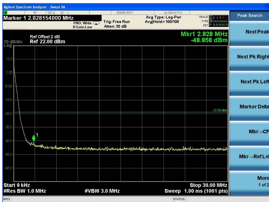
(Plot 4.9.2 A2: Channel 36: 5180MHz @ 802.11n HT20)
