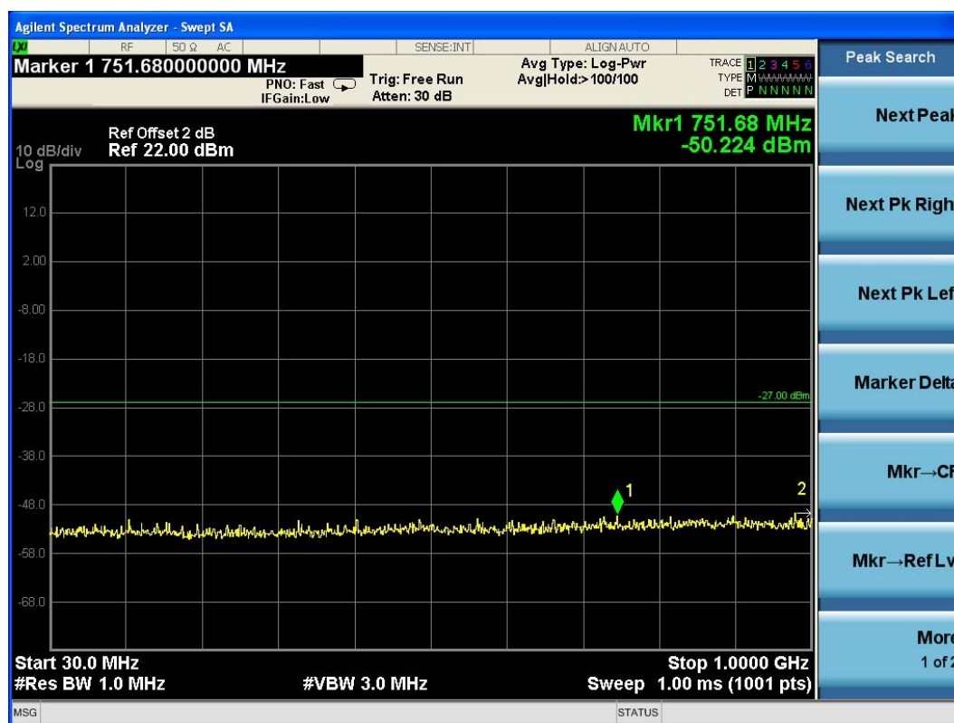
(Plot 4.9.2 B3: Channel 40: 5200MHz @ 802.11n HT20)
