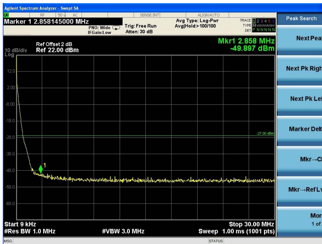
(Plot 4.9.1 C2: Channel 48: 5240MHz @ 802.11a)
