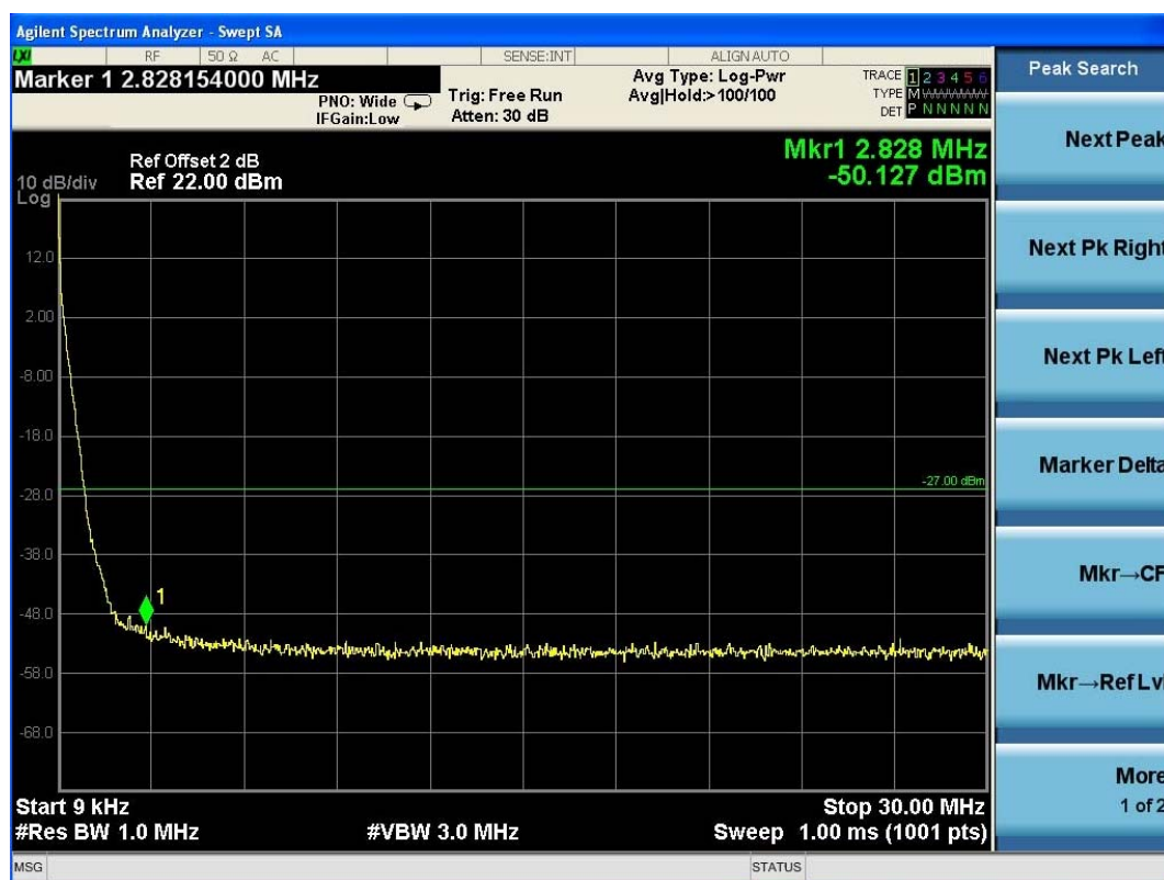
(Plot 4.9.2 C2: Channel 48: 5240MHz @ 802.11n HT20)
