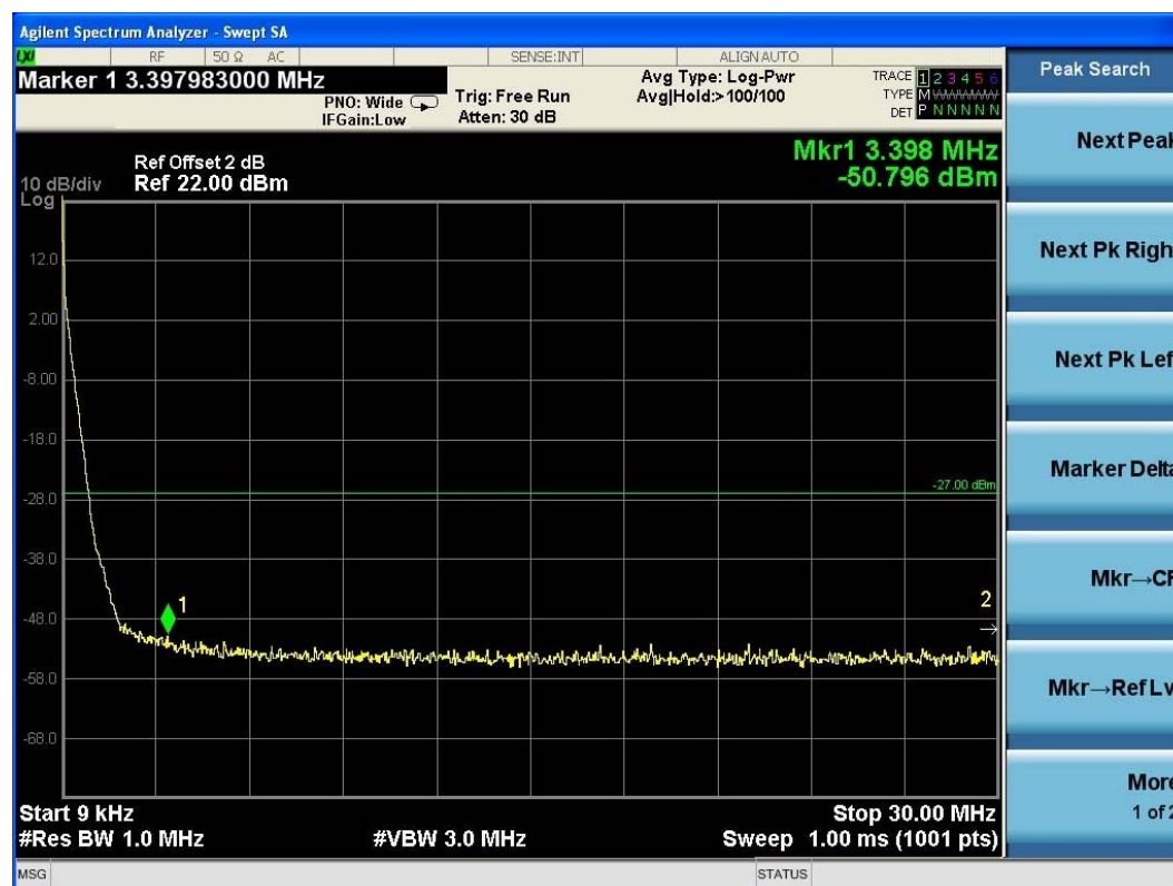
(Plot 4.9.2 B2: Channel 40: 5200MHz @ 802.11n HT20)
