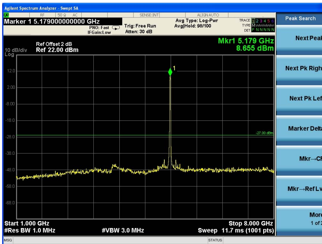
(Plot 4.9.1 A4: Channel 36: 5180MHz @ 802.11a)
