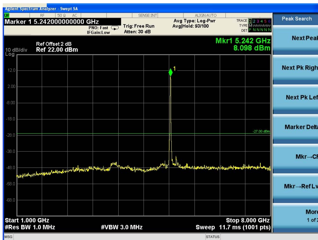
(Plot 4.9.1 C4: Channel 48: 5240MHz @ 802.11a)
