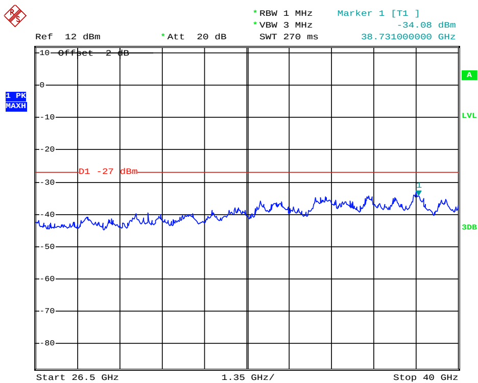
(Plot 4.9.2 B7: Channel 40: 5200MHz @ 802.11n HT20)
