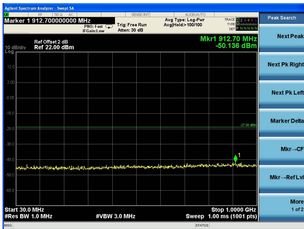
(Plot 4.9.2 C3: Channel 48: 5240MHz @ 802.11n HT20)
