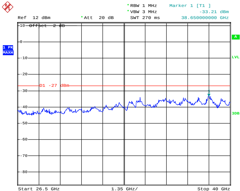
(Plot 4.9.2 A7: Channel 36: 5180MHz @ 802.11n HT20)
