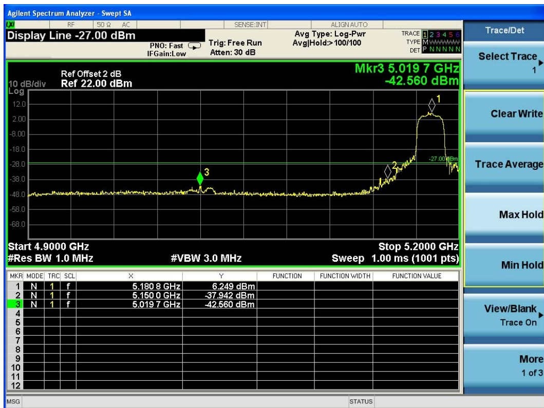
(Plot 4.9.2 A1: Channel 36: 5180MHz @ 802.11n HT20)
