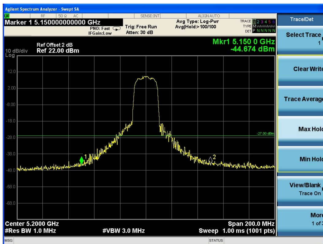
(Plot 4.9.2 B1: Channel 40: 5200MHz @ 802.11n HT20)
