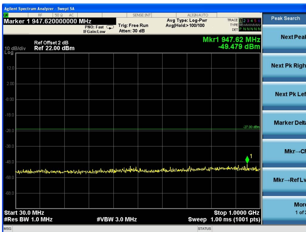
(Plot 4.9.1 A3: Channel 36: 5180MHz @ 802.11a)
