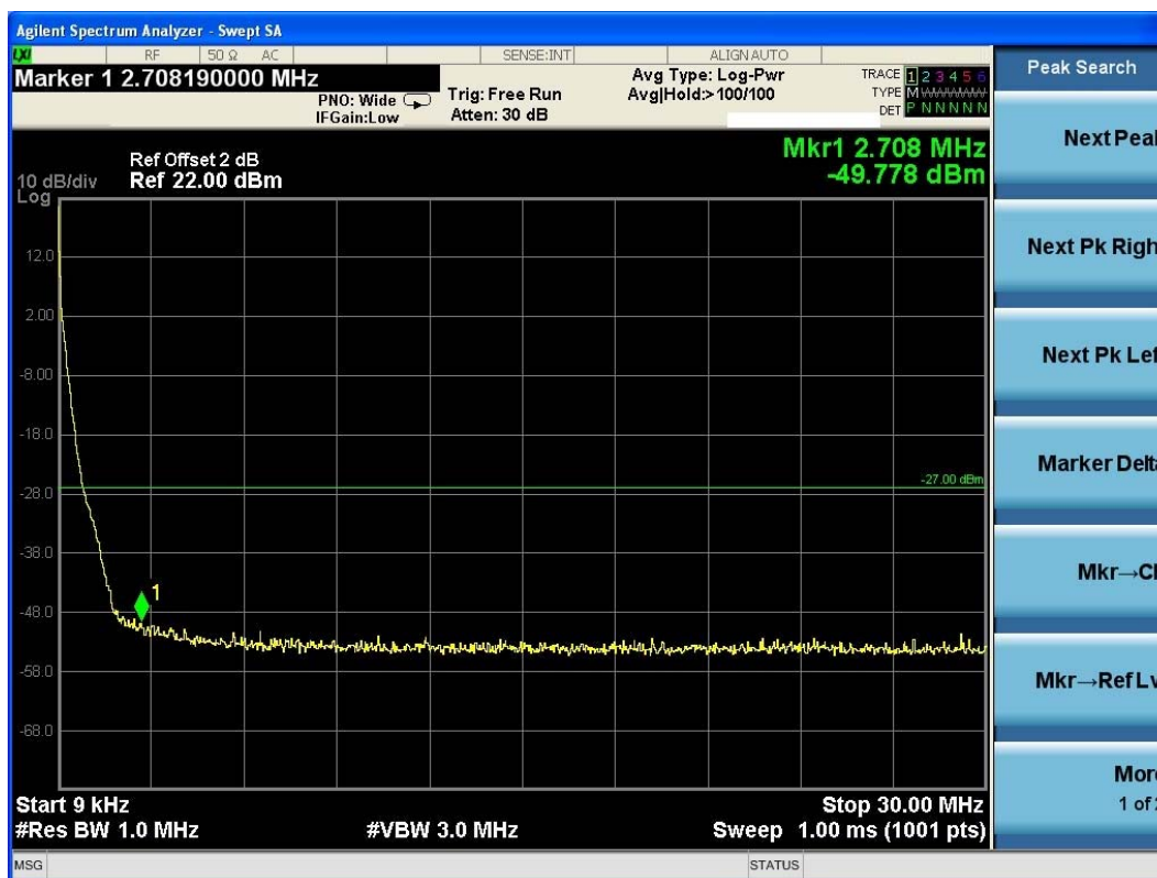
(Plot 4.9.1 A2: Channel 36: 5180MHz @ 802.11a)
