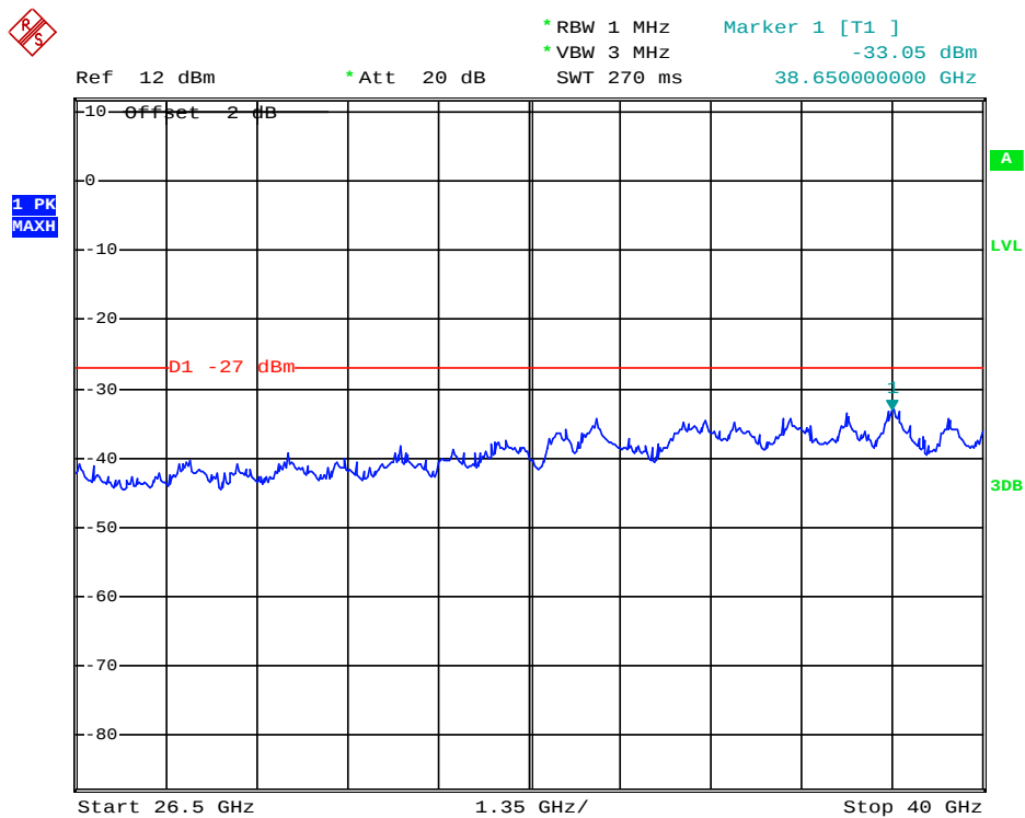
(Plot 4.9.1 C7: Channel 48: 5240MHz @ 802.11a)
