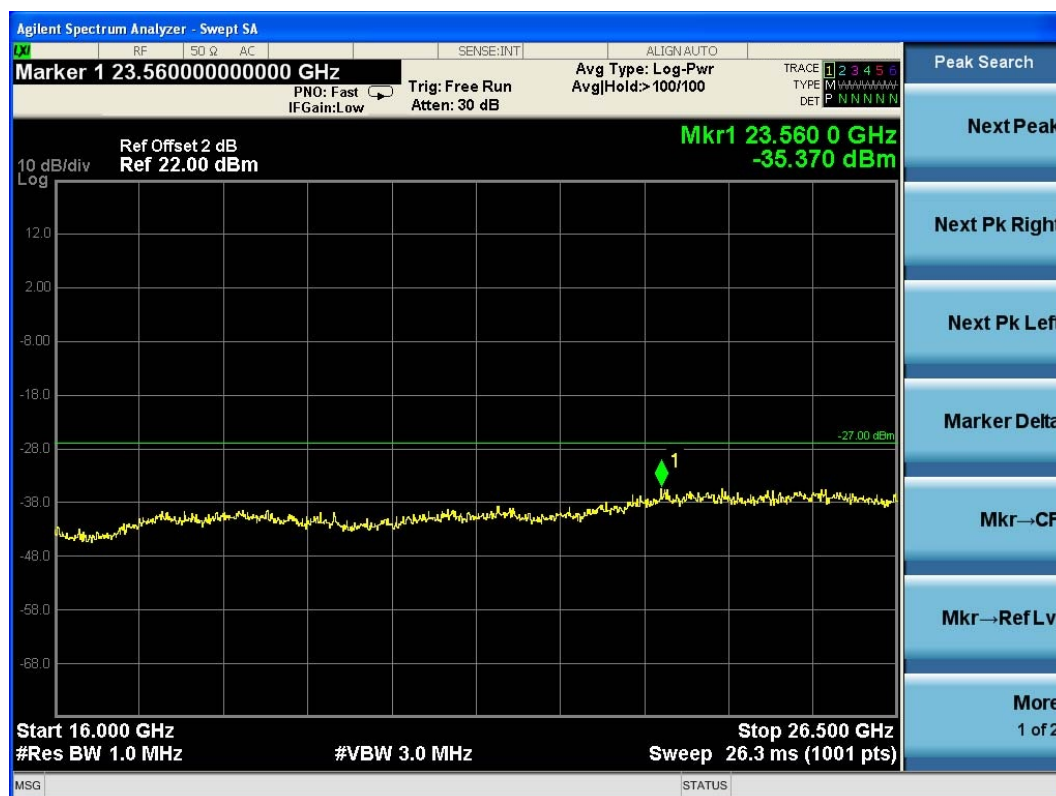
(Plot 4.9.2 B6: Channel 40: 5200MHz @ 802.11n HT20)
