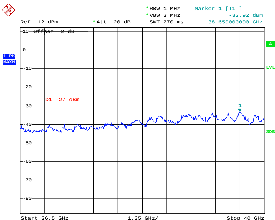
(Plot 4.9.1 A7: Channel 36: 5180MHz @ 802.11a)
