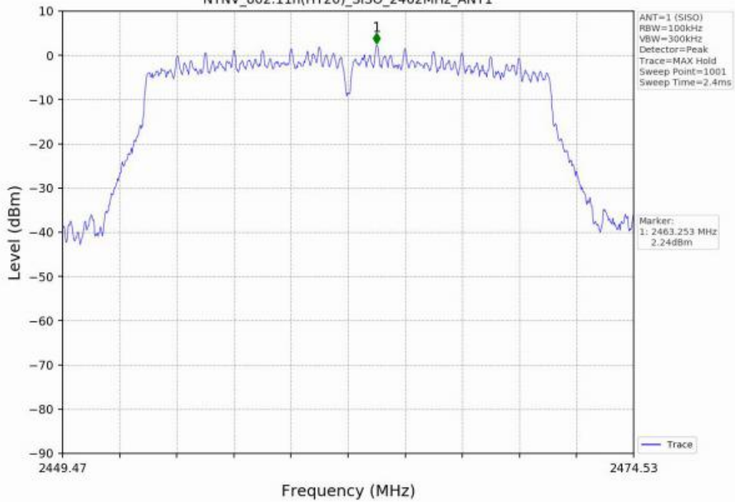
Unwanted Emissions in Non-restricted Frequency Bands NTNV_802.11n(HT20)_SISO_2462MHz_ANT1
