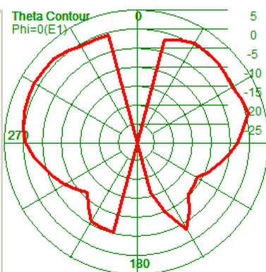
Peak Gain: 3.44dBi
