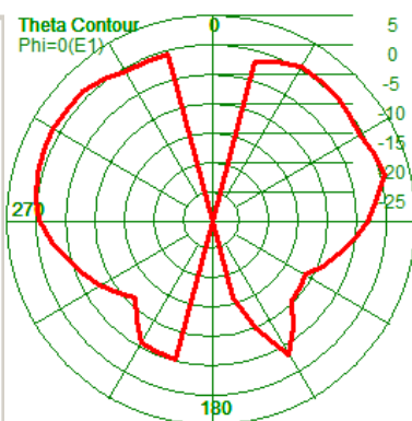
Peak Gain: 3.30dBi
