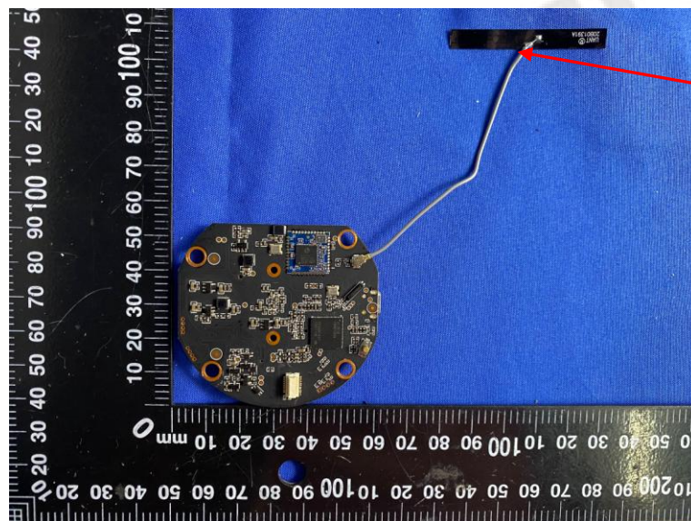
WIFI Antenna
