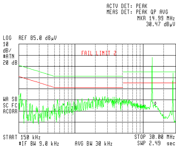
Figure 5. Detectors: Peak, Quasi-peak, Average
