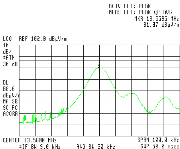
Figure 8. Field Strength of Fundamental Detector: Peak
