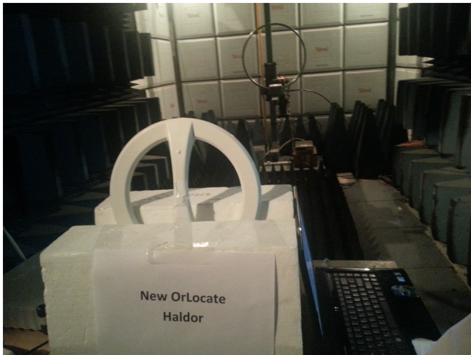
Screening, Fundamental, and Radiated Emission Test 9kHz-30MHz Locator
