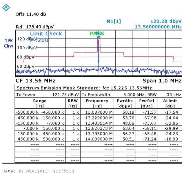
Figure 22. Mask of Fundamental, Locator Antenna
