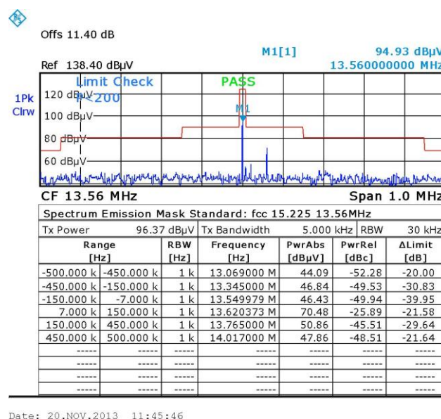
Figure 20. Mask of Fundamental Tool Add Antenna
