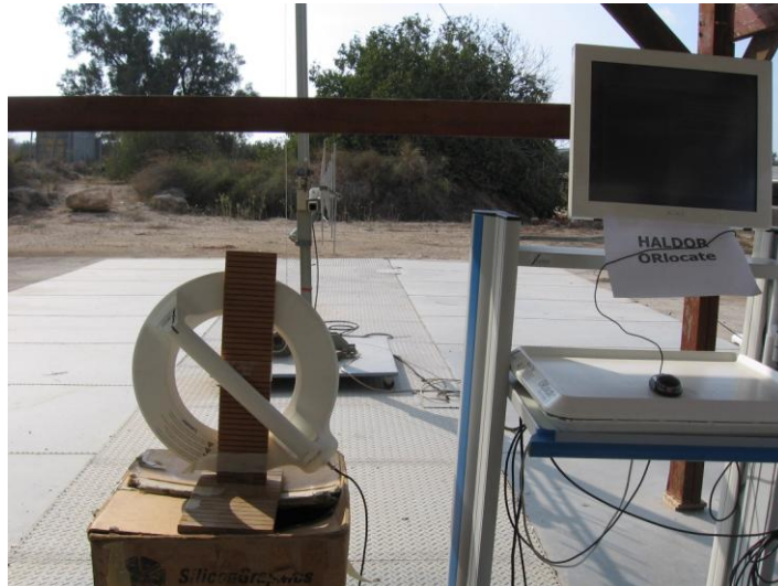
Figure 12. Radiated Emission Test 300MHz-1000MHz Locator
