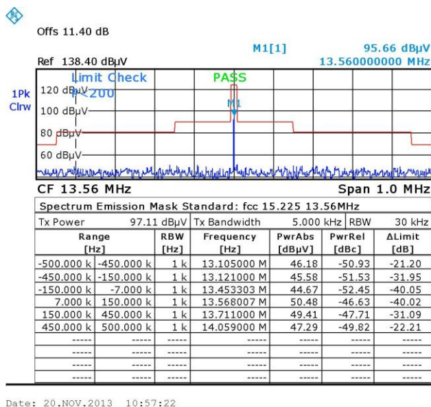
Figure 24. Mask of Fundamental Flat Antenna
