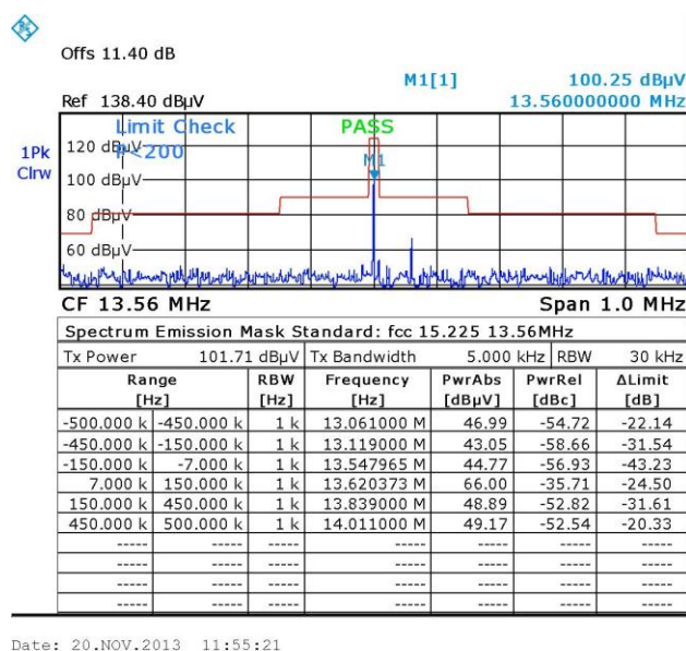
Figure 18. Mask of Fundamental Sponge Bucket Antenna
