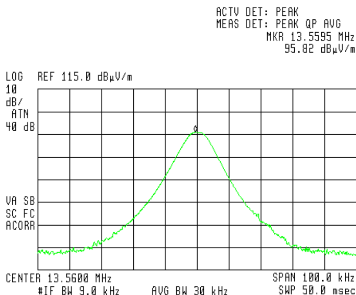
Figure 23. Field Strength of Fundamental, Flat Antenna
