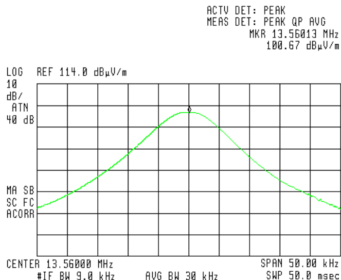
Figure 17. Field Strength of Fundamental, Sponge Bucket Antenna
