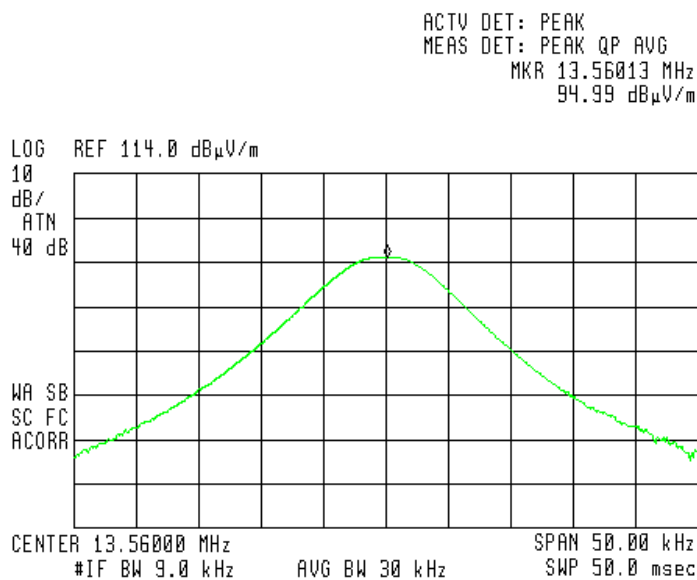
Figure 19. Field Strength of Fundamental, Tool Add Antenna
