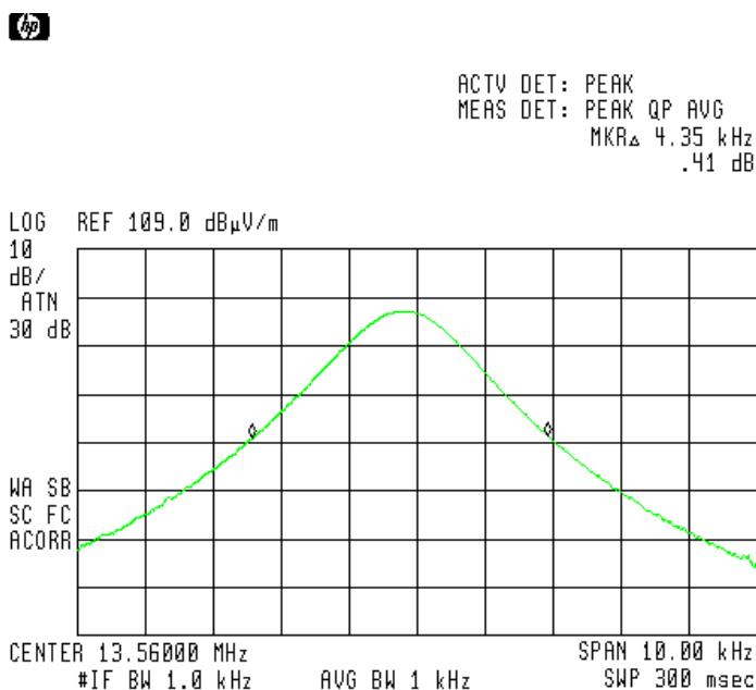
Figure 14. 13.56 MHz
