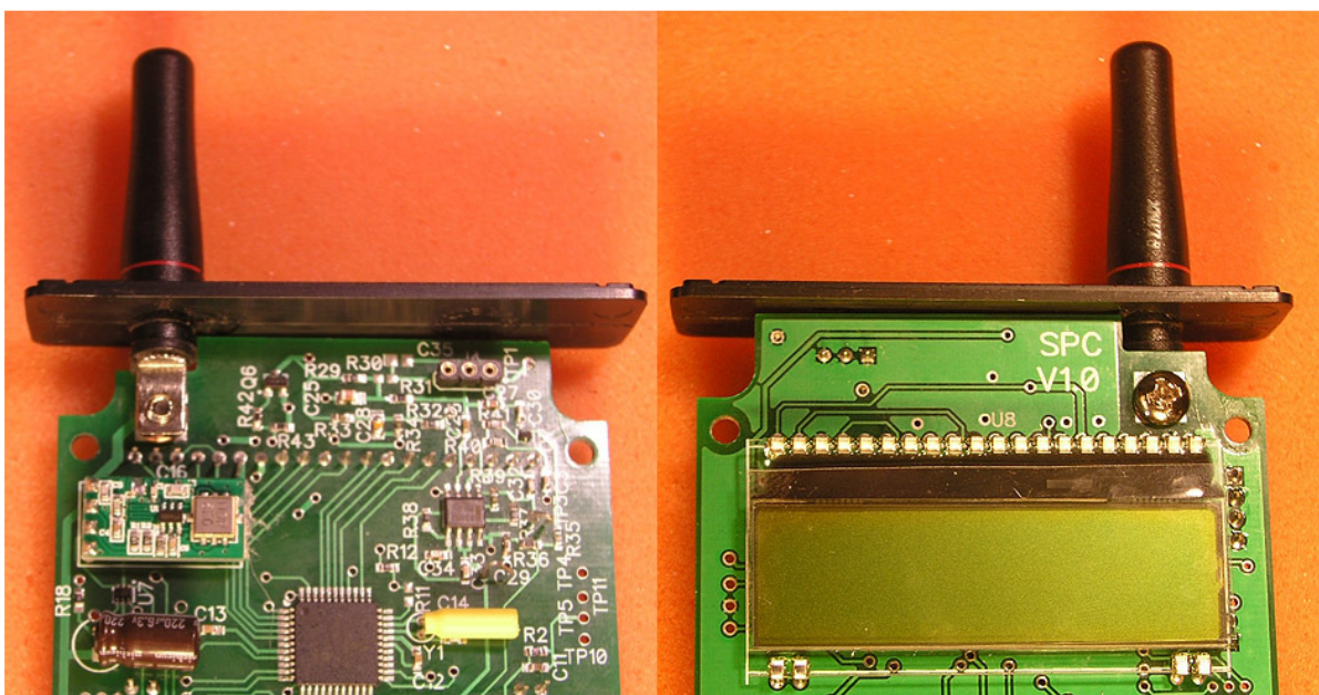
P.C. Board close-up on RF and fixed antenna areas Top view Bottom view showing antenna screw
