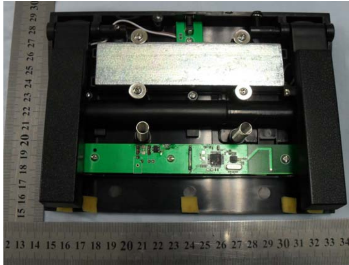
EUT - PCB View of TX part
