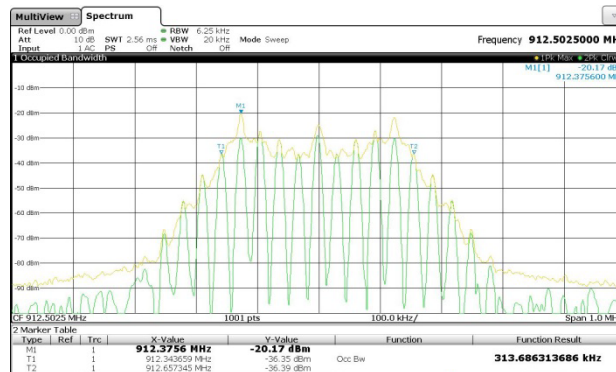
Occupied Bandwidth – lowest channel
