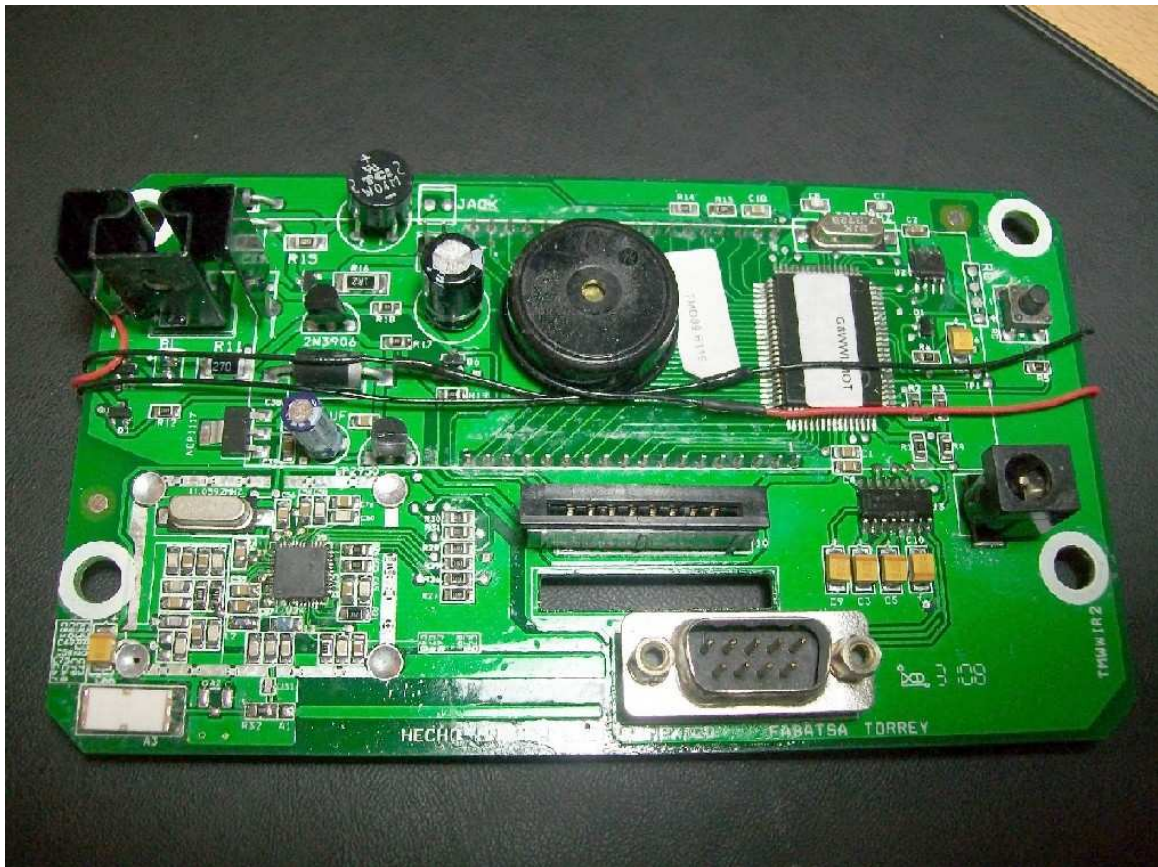
Receiver PCB photo – top side
