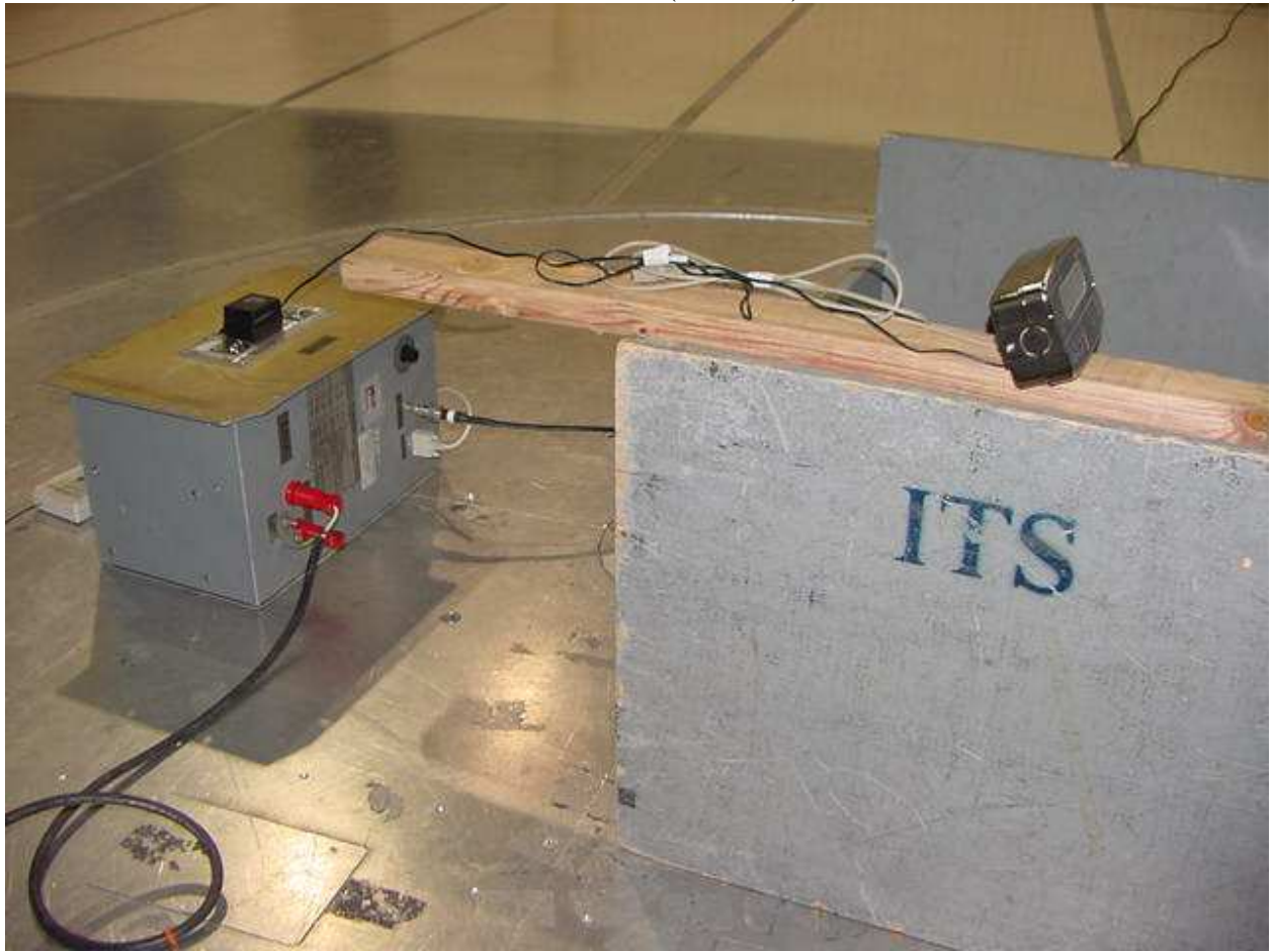
Conducted Emissions (Receiver)
