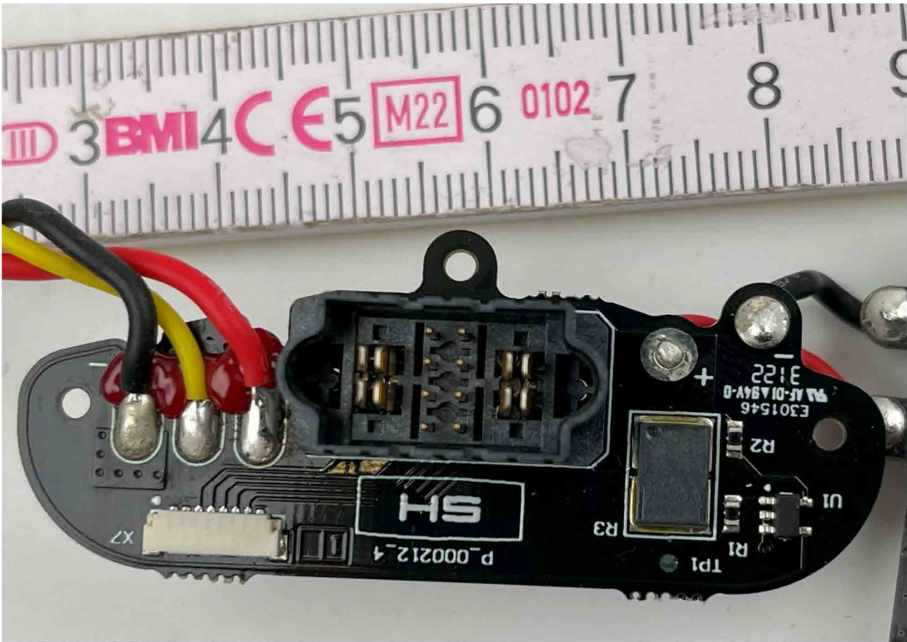
Male Battery board:
