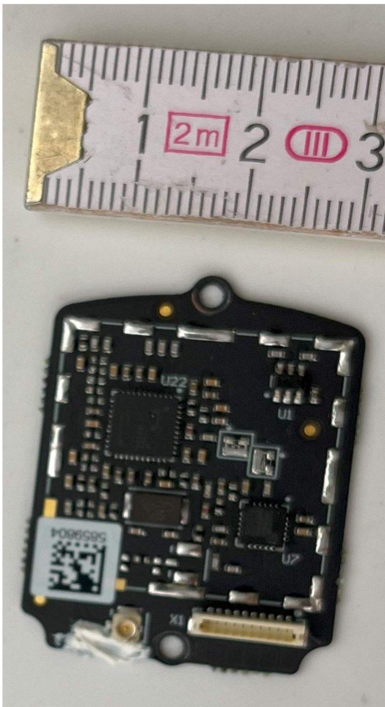
VTX board
