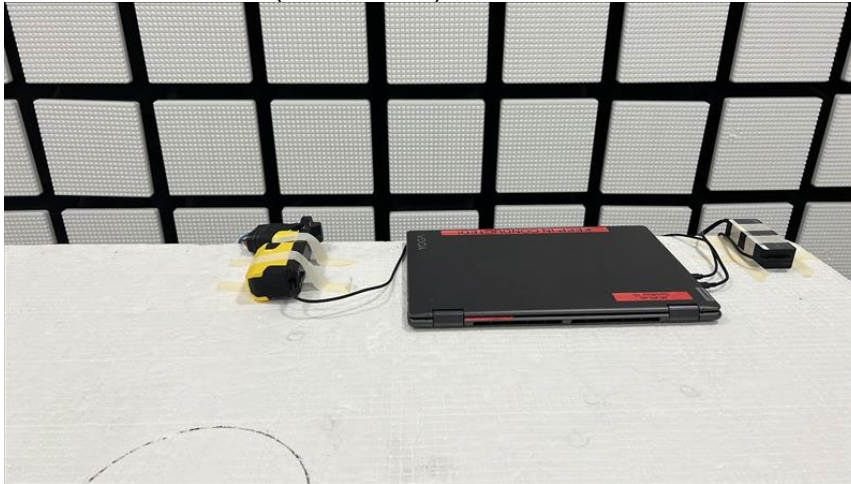
RADIATED PHOTO (>1000 MHz)
