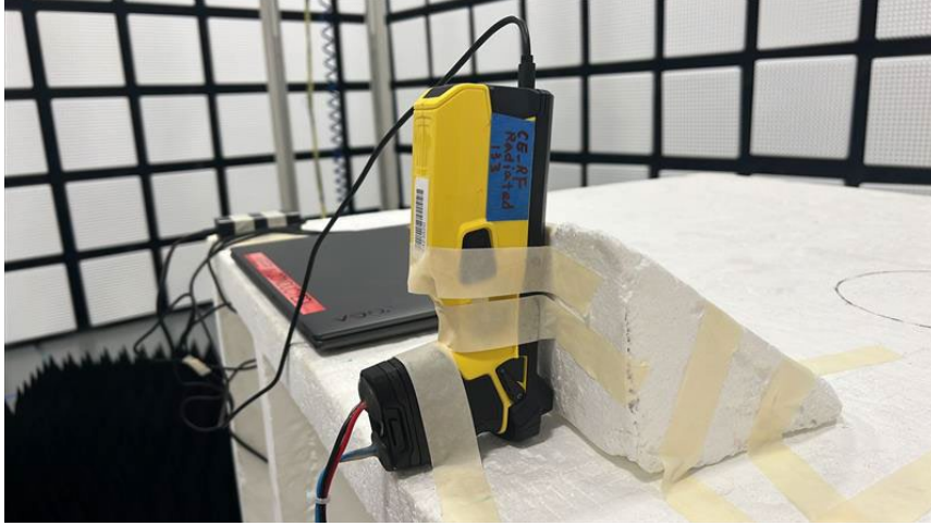
Z-ORIENTATION
