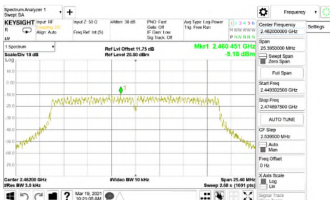
Power Density_802.11n_20MHz_Chain0_2462MHz
