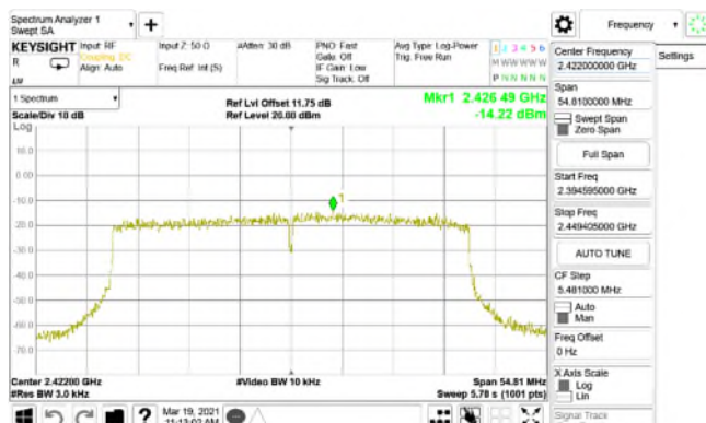
Power Density_802.11ax_40MHz_Chain0_2422MHz_RU242_61
