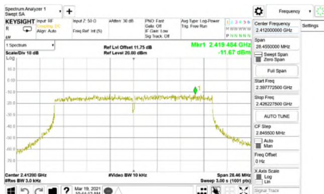
Power Density_802.11ax_20MHz_Chain0_2412MHz_RU106_53
