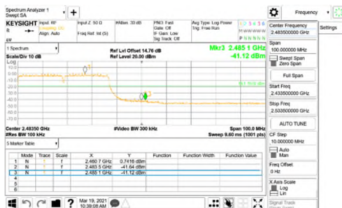
Bandedge_802.11n_40MHz_Chain0_2452MHz
