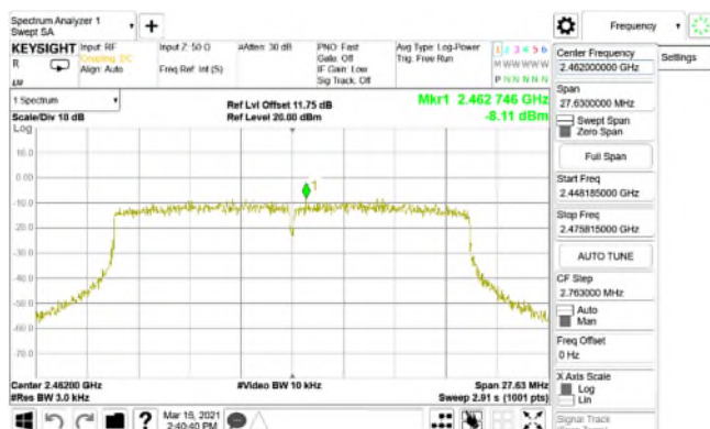
Power Density_802.11ax_20MHz_Chain0_2462MHz
