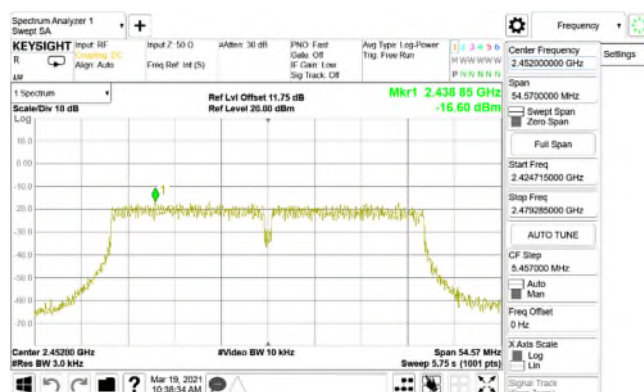
Power Density_802.11n_40MHz_Chain1_2452MHz
