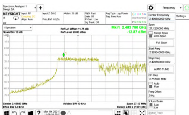
Power Density_802.11ax_20MHz_Chain0_2412MHz_RU26_0
