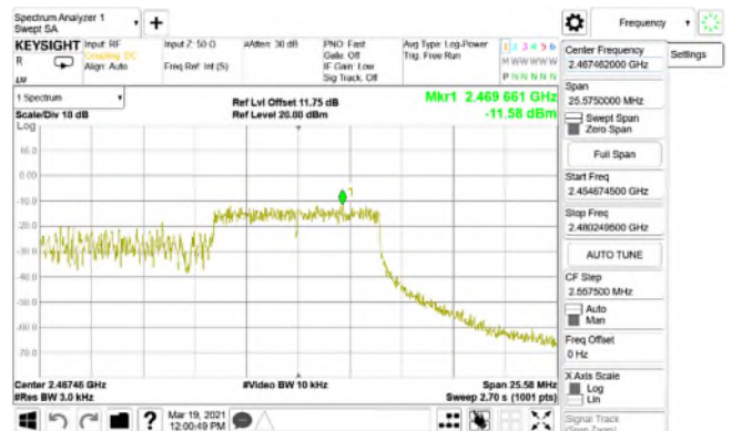
Power Density_802.11ax_20MHz_Chain1_2462MHz_RU26_8
