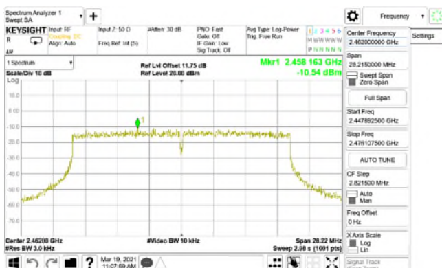
Power Density_802.11ax_20MHz_Chain1_2462MHz
