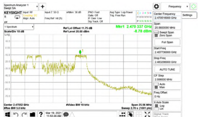
Power Density_802.11ax_20MHz_Chain1_2462MHz_RU52_40
