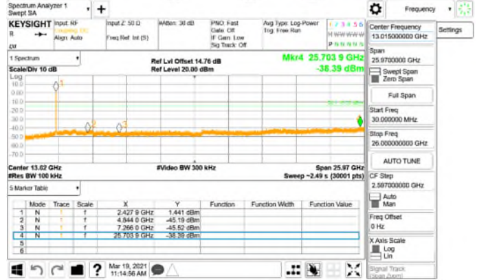
Spurious Emission_802.11ax_40MHz_Chain0_2437MHz
