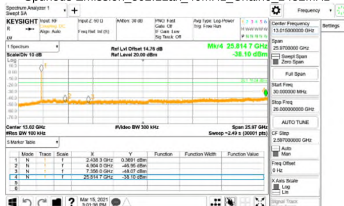
Spurious Emission_802.11ax_40MHz_Chain0_2452MHz
