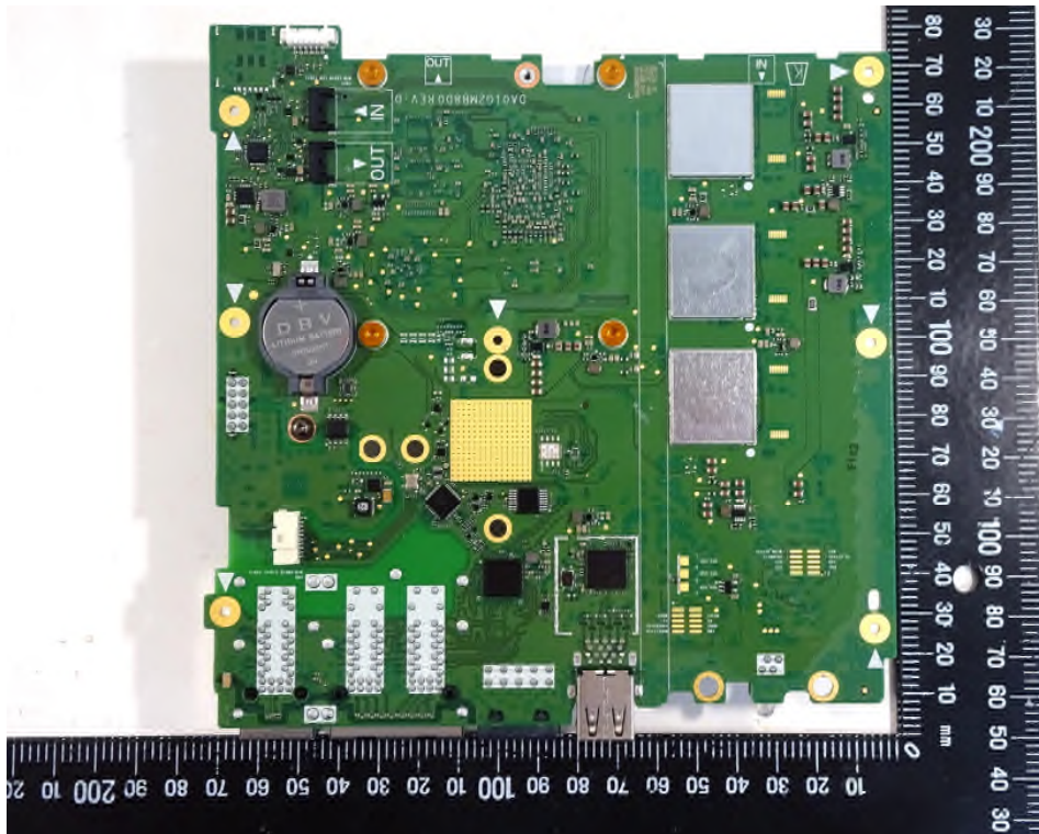
Internal View of EUT –3
