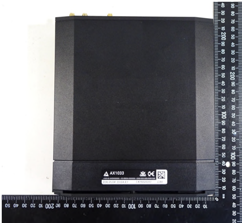
Front View of EUT
