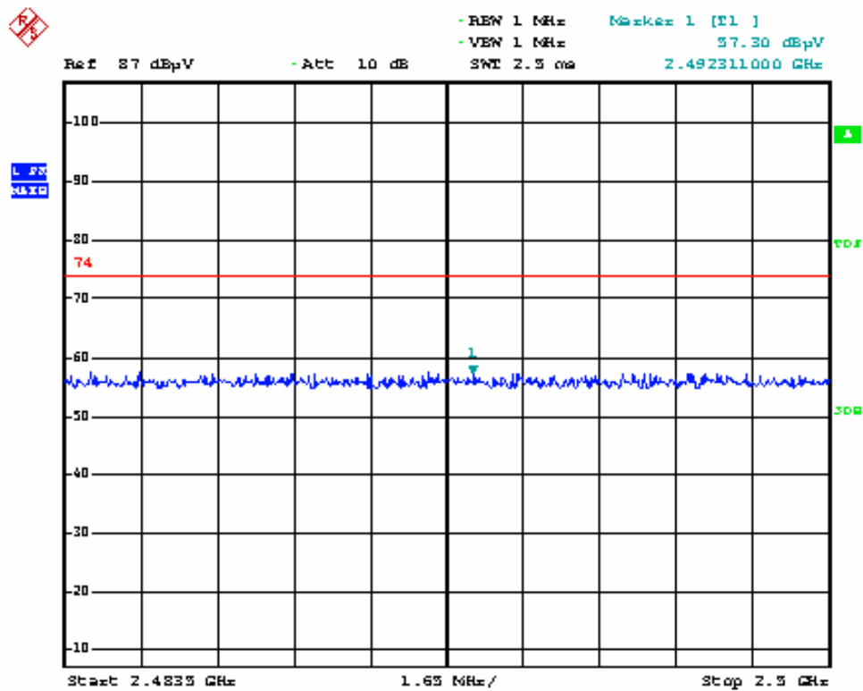
802.11n-40MHz high channel Hor Peak
