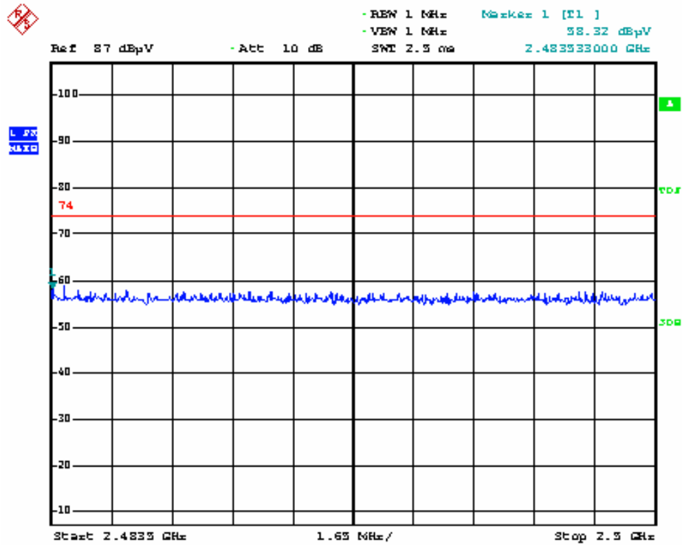
802.11n-20MHz high channel Hor Peak
