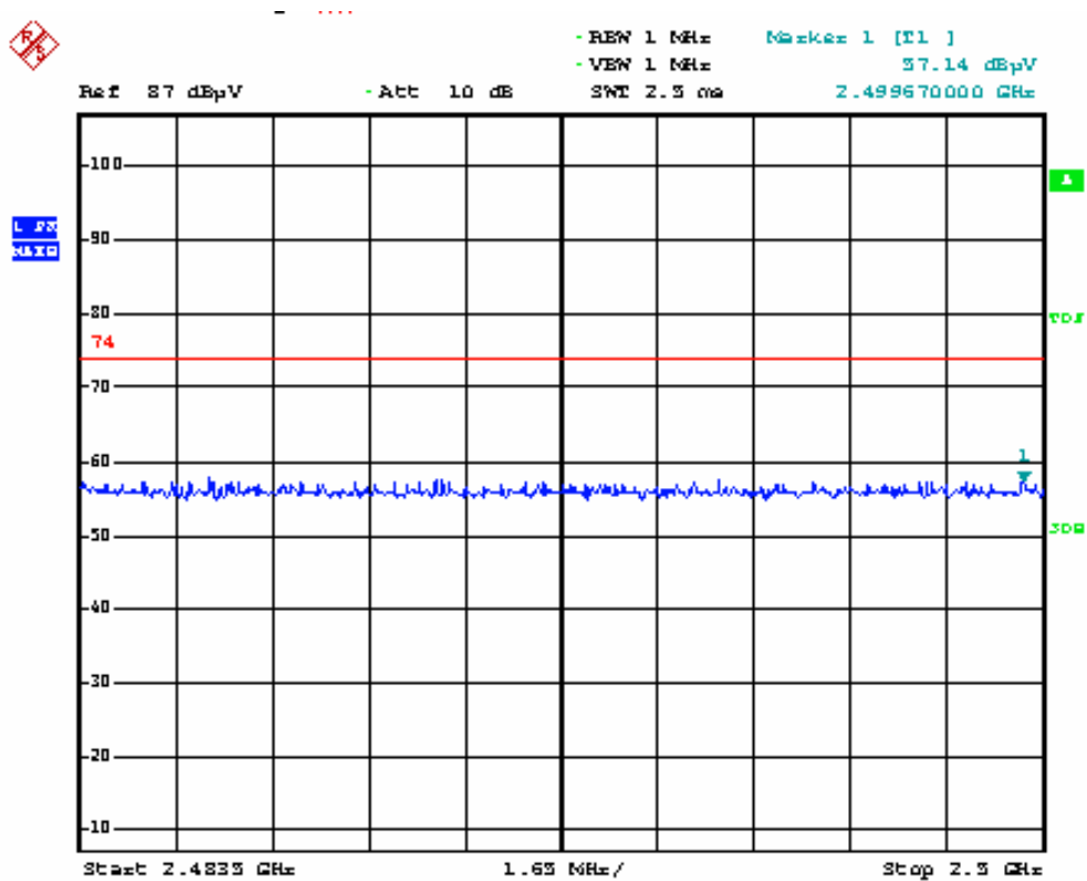
802.11n-20MHz high channel Ver Peak
