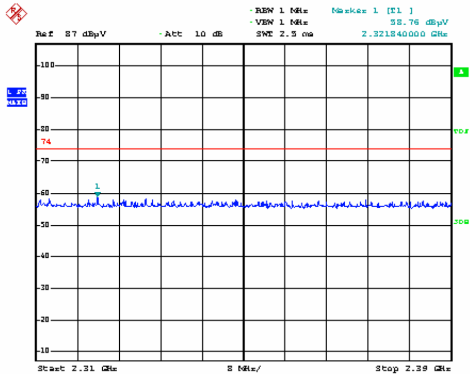
802.11b low channel Hor Peak
