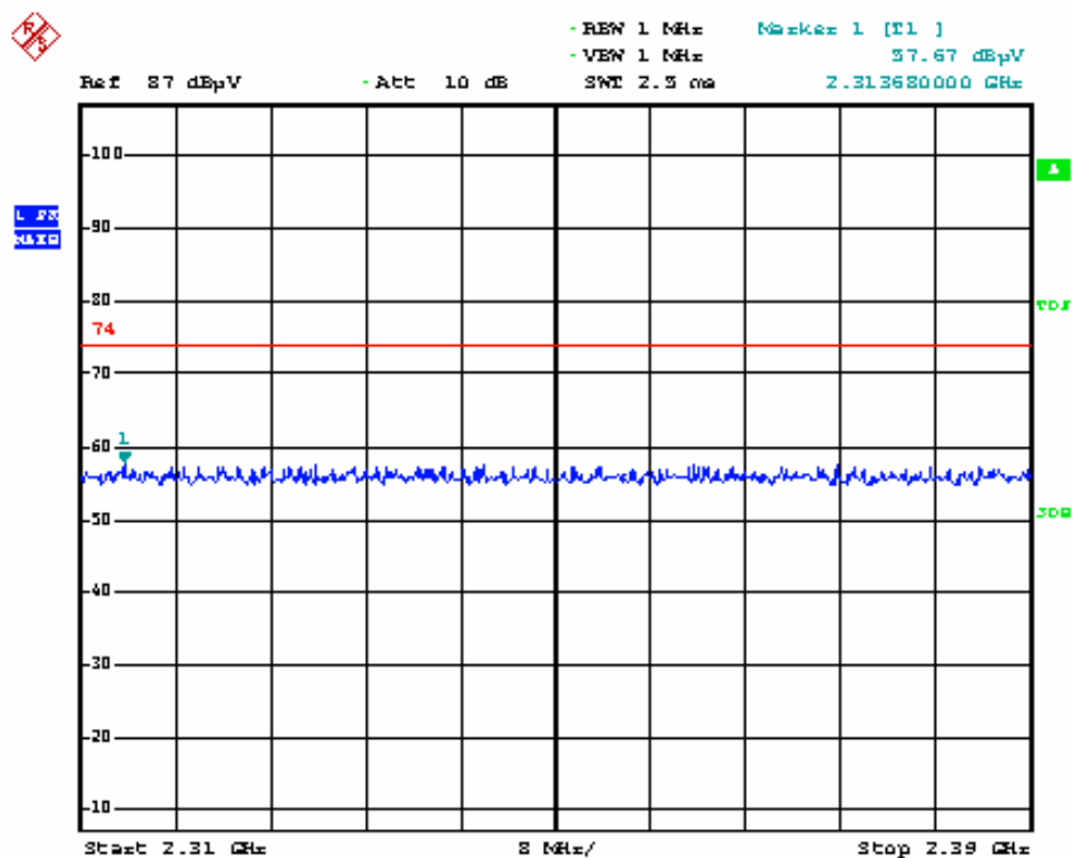
802.11n-20MHz low channel Hor Peak
