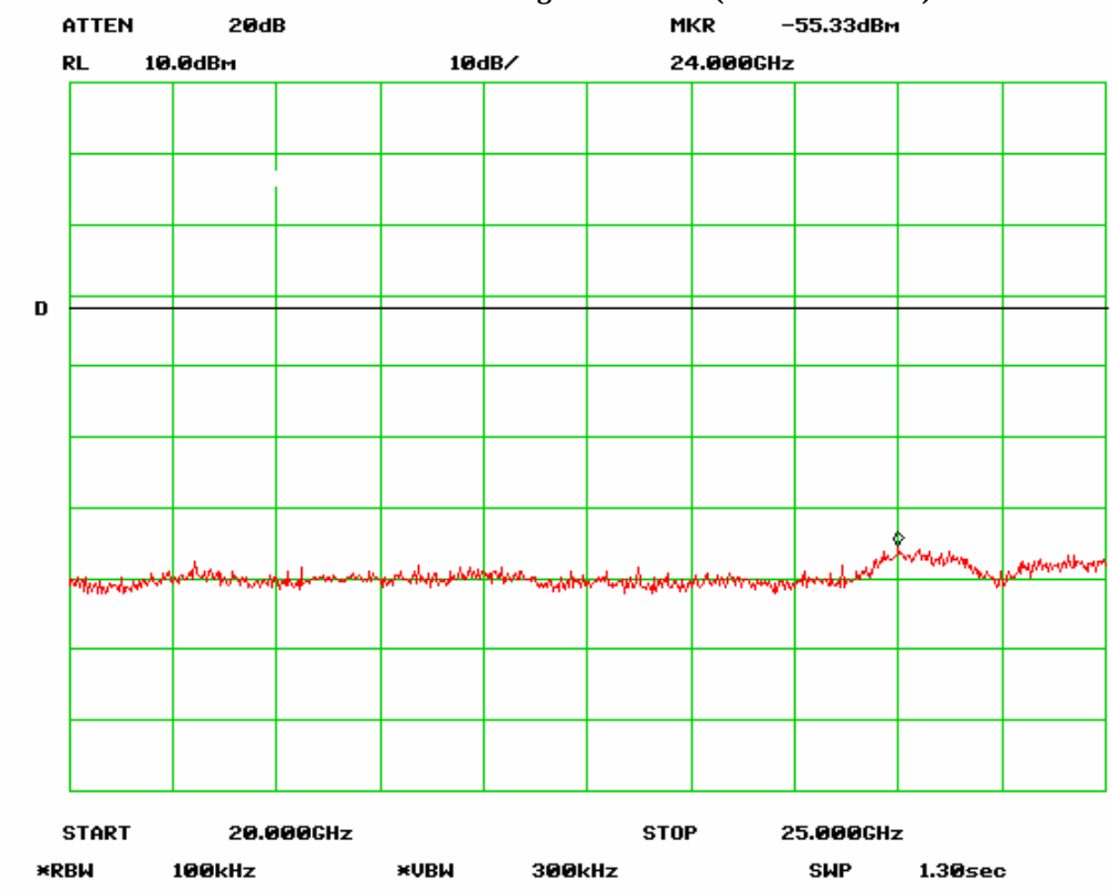
Antenna Port Emission High-6 Channel (802.11n 40MHz)
