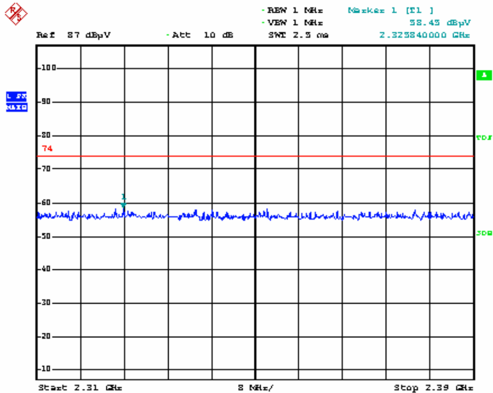
802.11n-20MHz low channel Ver Peak
