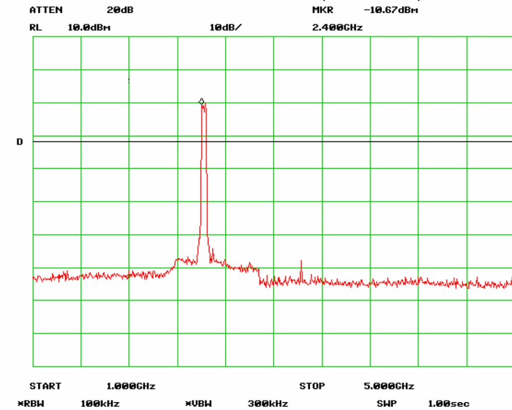
Antenna Port Emission Low-2 Channel (802.11n 40MHz)
