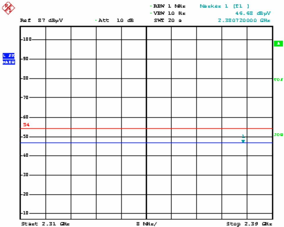
802.11n-40MHz low channel Hor Peak
