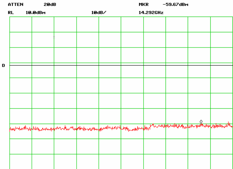
Antenna Port Emission Low-3 Channel (802.11n 40MHz)
