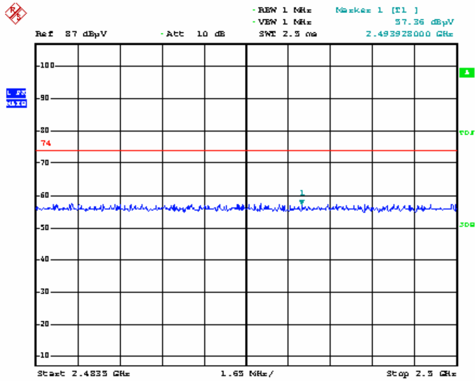
802.11b high channel Ver Peak
