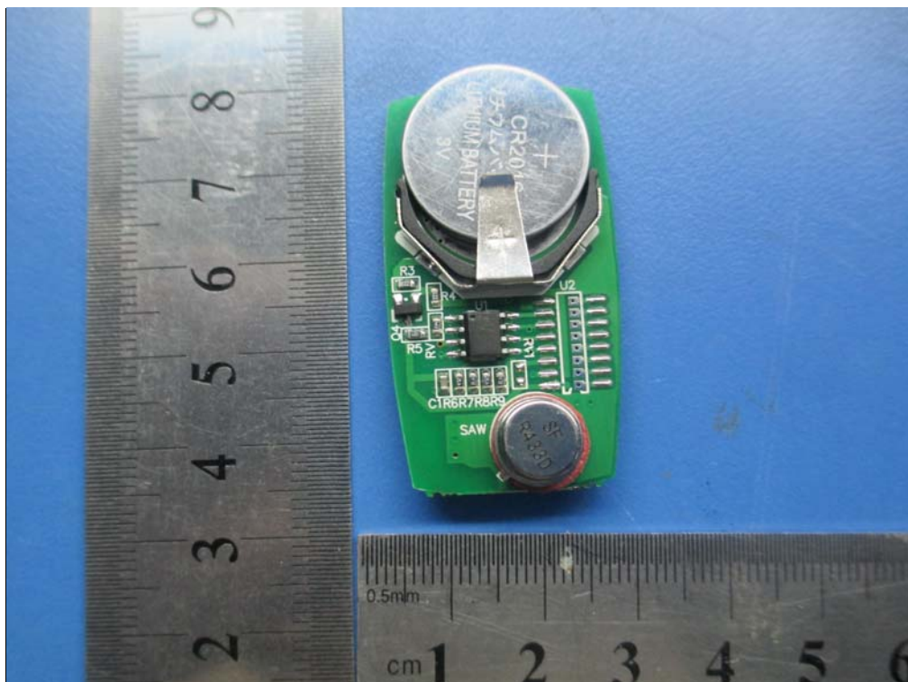
EUT (Transmitter) – PCB 1 Front View
