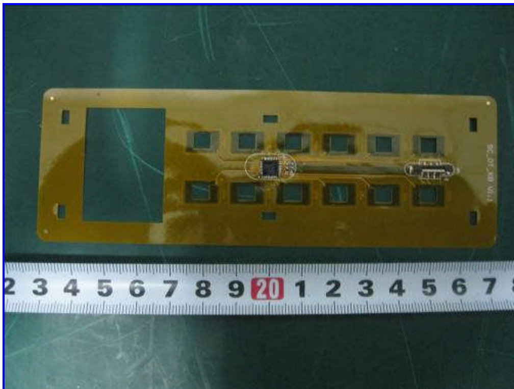
Front View of Keyboard PCB Board
