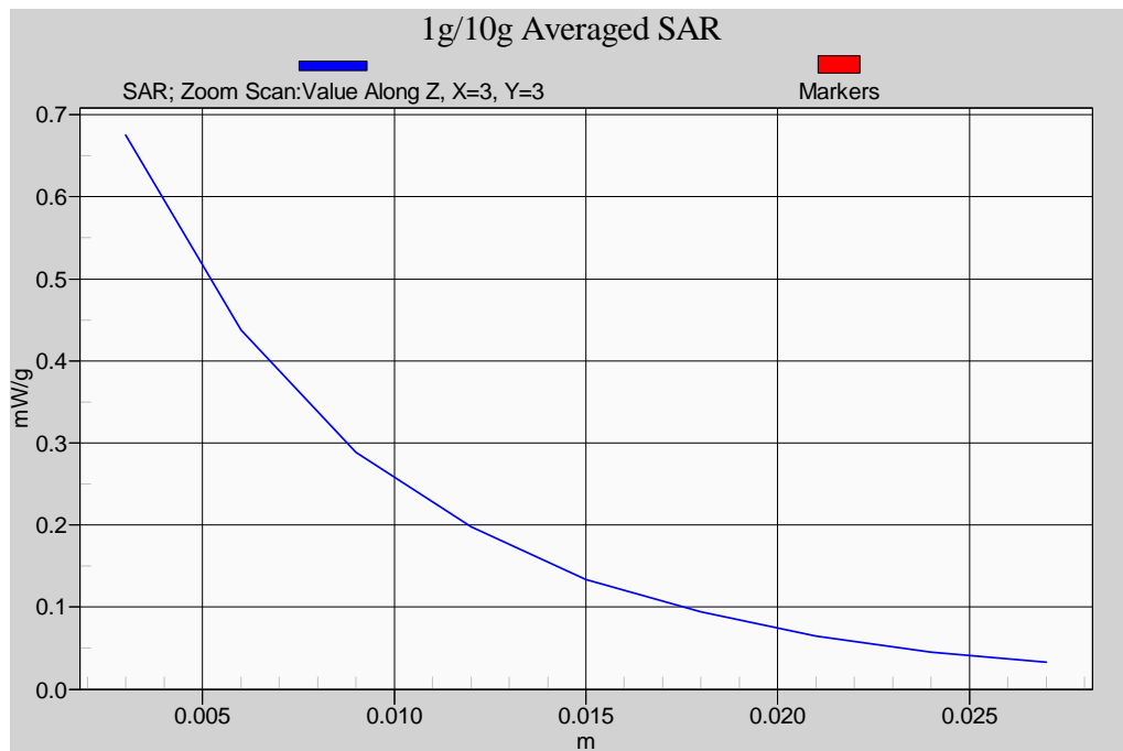
Z-axis Plot of Flat WLAN 802.11n_HT40 CH 6 (Rate 130M)
