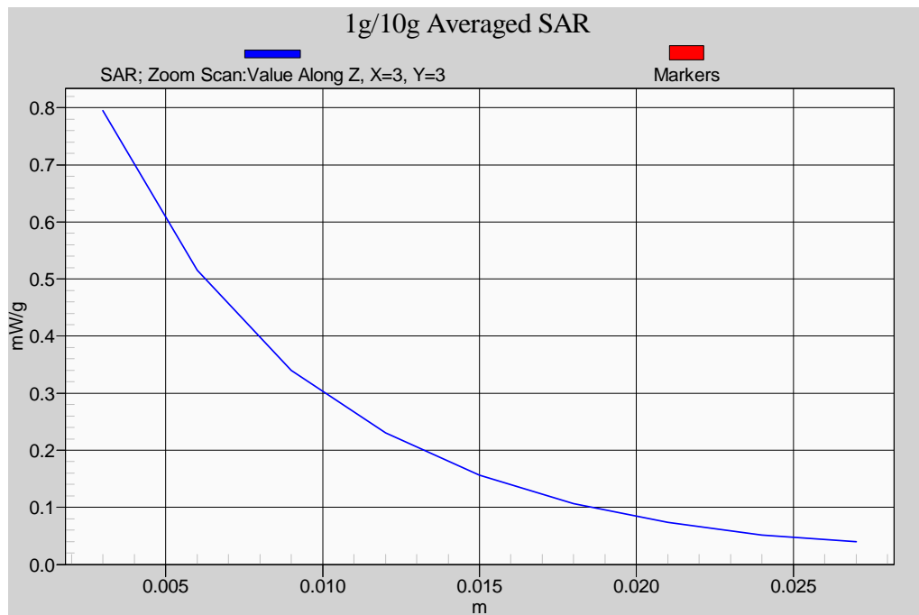
Z-axis Plot of Flat WLAN 802.11n_HT20 CH 11 (Rate 52M)
