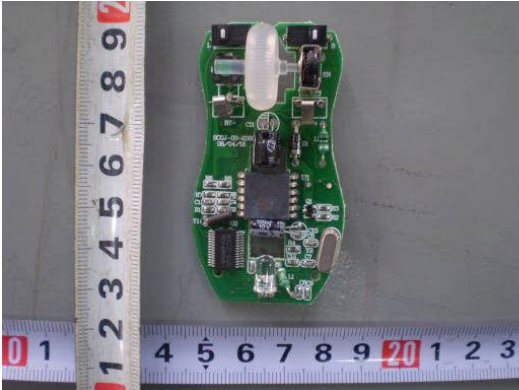
Top View of mouse PCB
