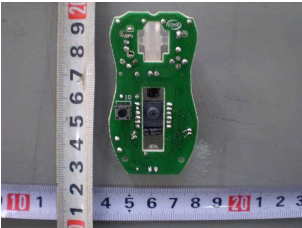
Bottom View of mouse PCB
