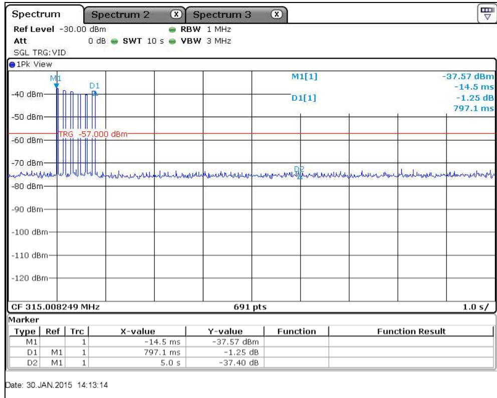
Figure 7.3.2-1: TX Hold Time
