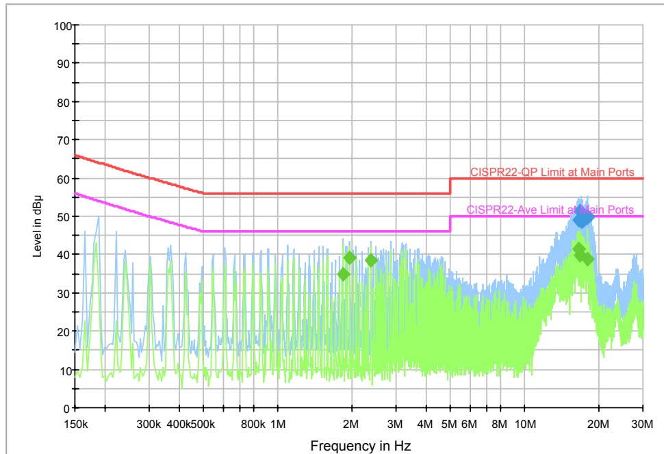
EMI_ENV216 Auto Test-L CISPR22
