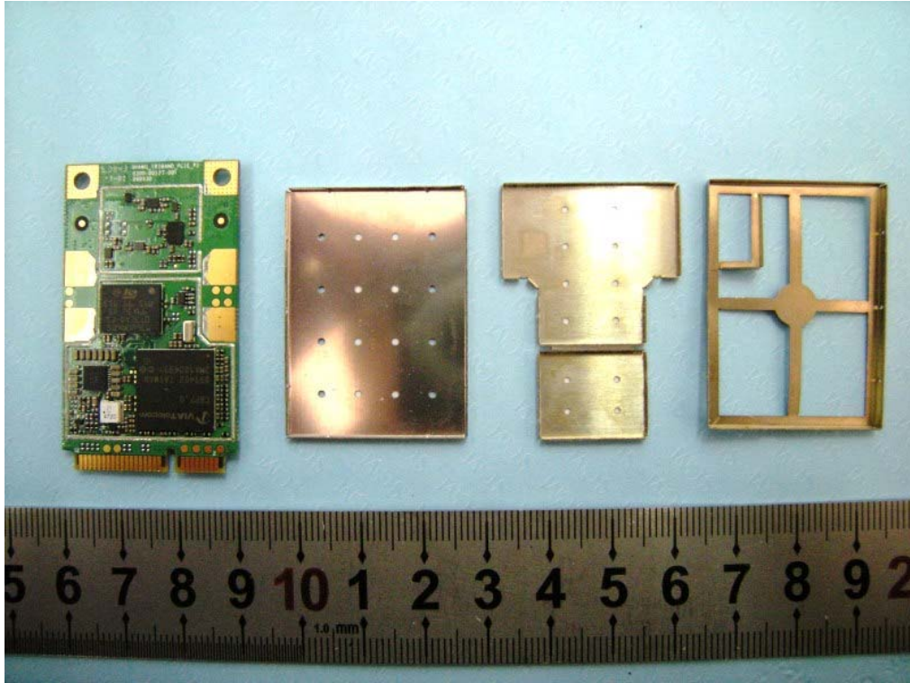
EUT & SHIELDING
