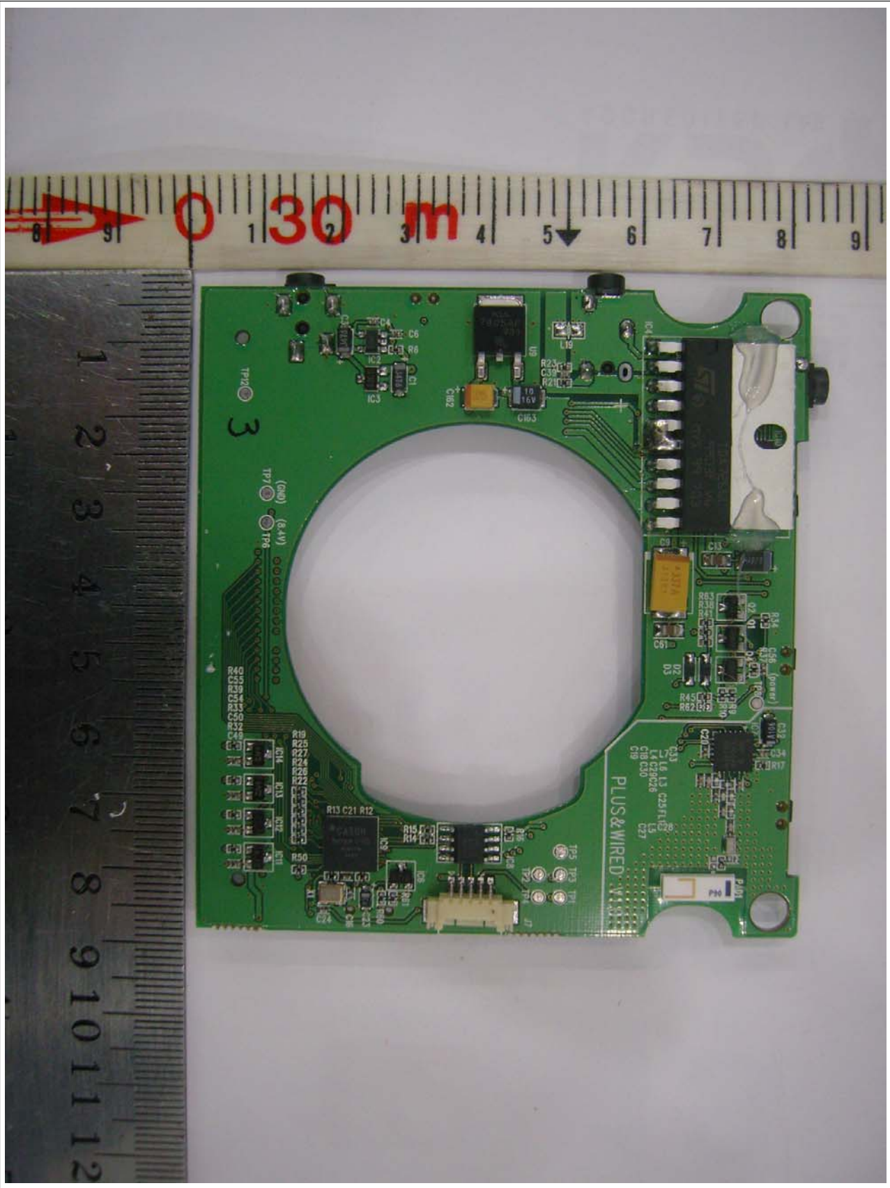
View of Main PCB
