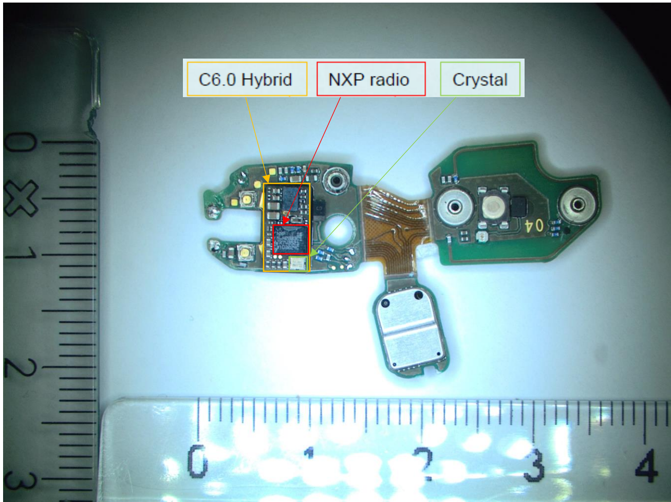
Top (main PCBA)
