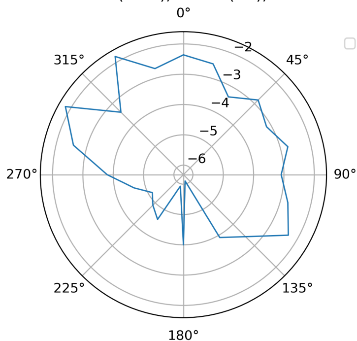
Total EIRP (dBm), Phi=0 (XZ), f=2440
