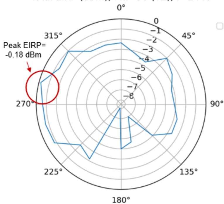
Total EIRP (dBm), Phi=90 (YZ), f=2440
