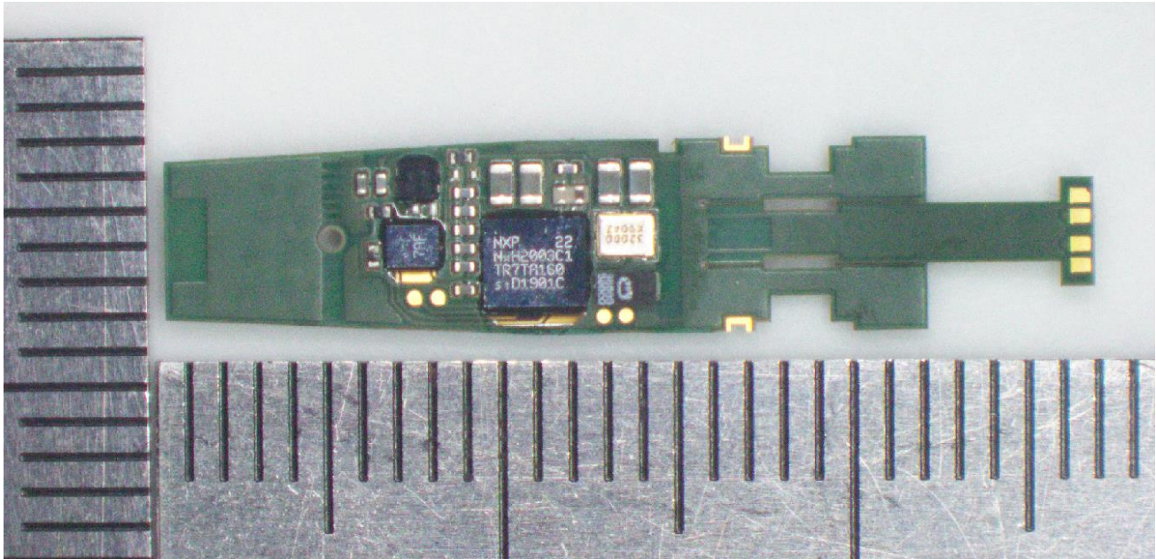
PCB BOTTOM SIDE VIEW
