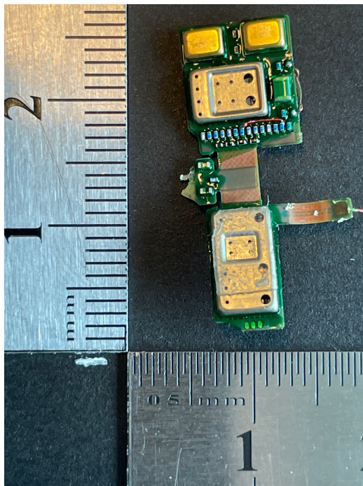
PCBA TOP SIDE VIEW
