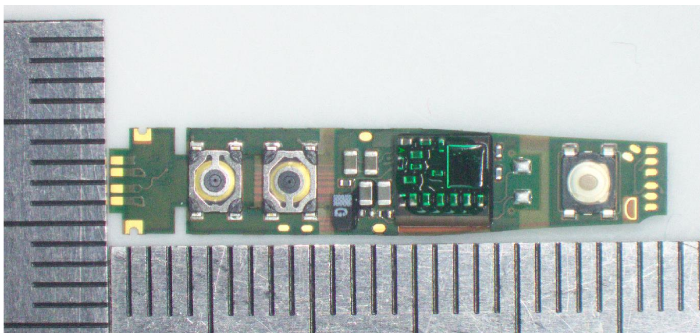
PCB TOP SIDE VIEW
