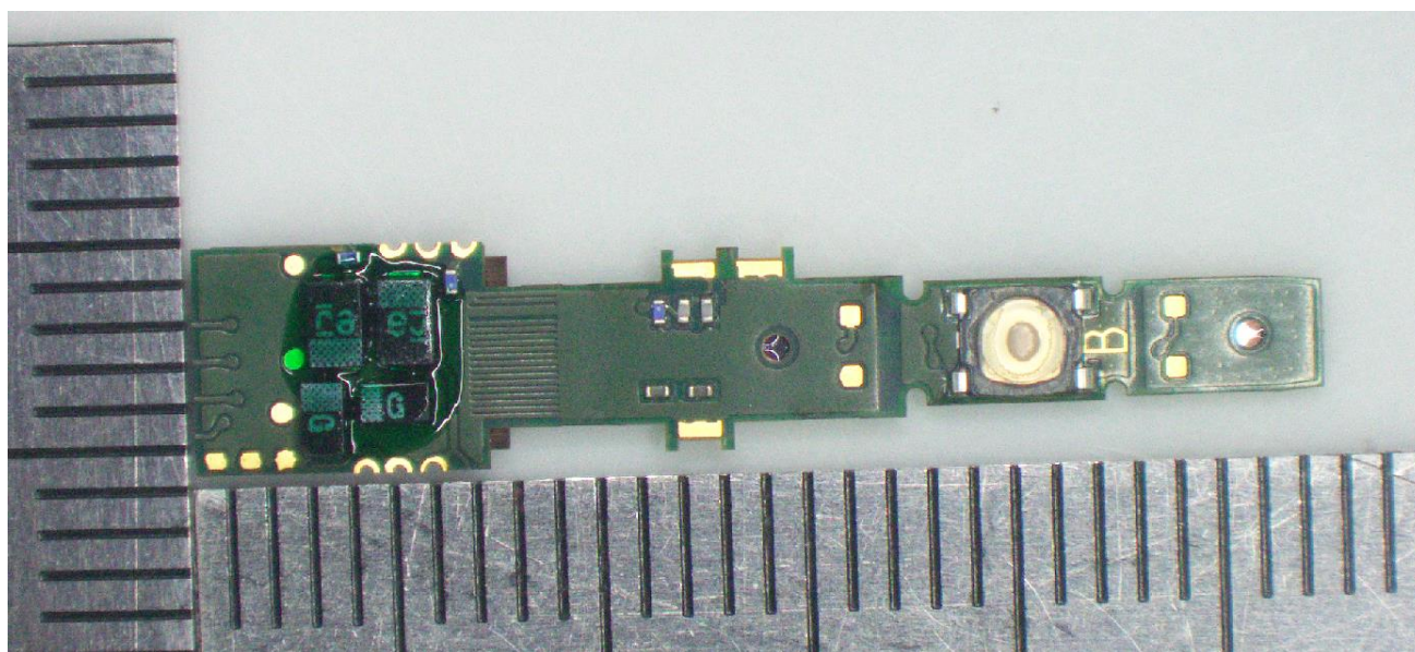
PCB TOP SIDE
