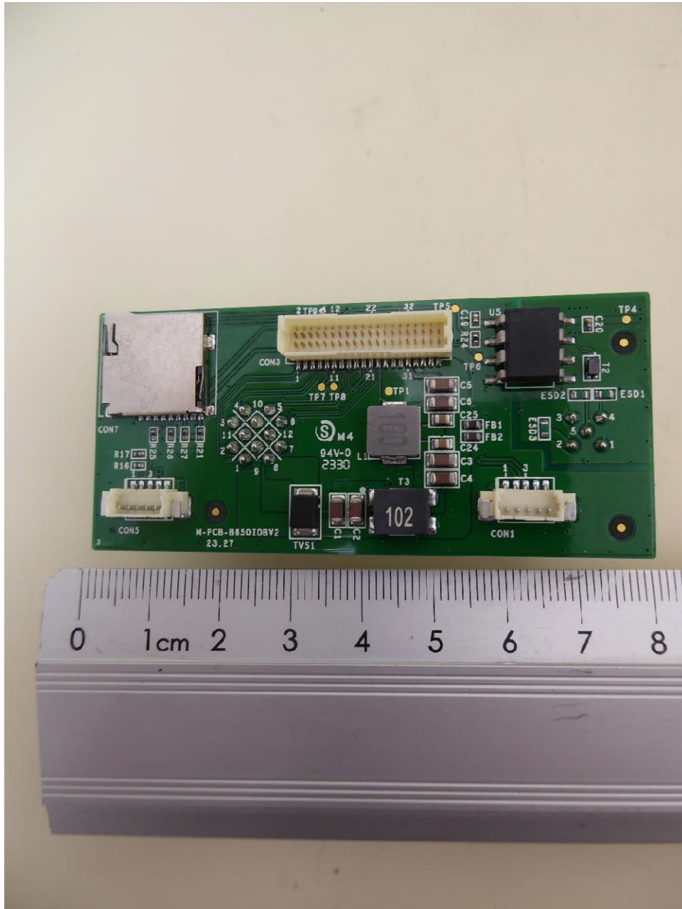
B650S / B650WS, connector PCB, bottom view
