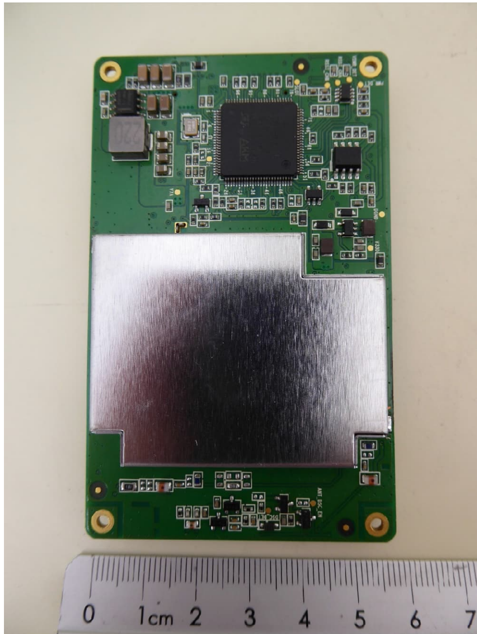
B650S / B650WS, main PCB, bottom view
