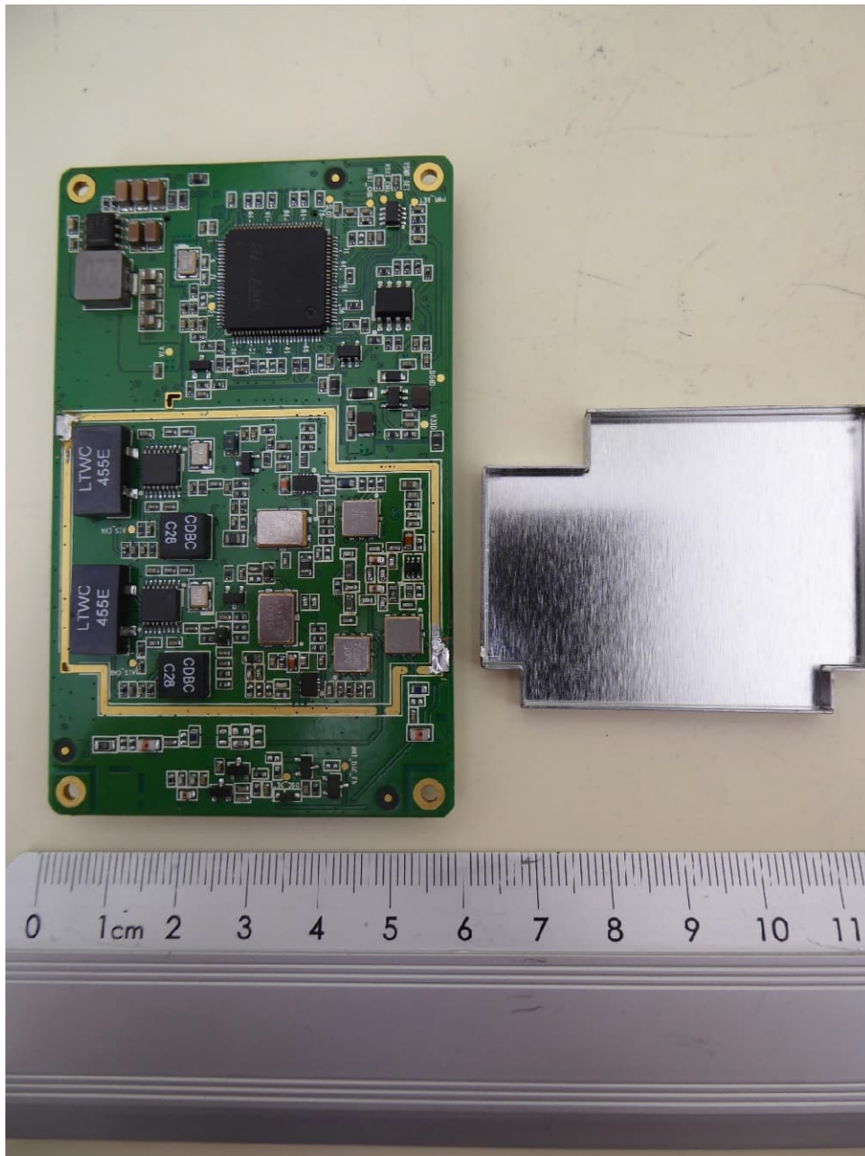
B650S / B650WS, main PCB, bottom view, shielding removed
