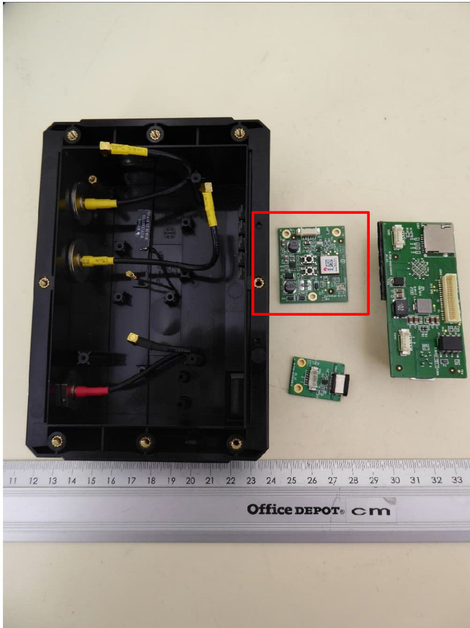
B650WS (with certified Wifi Module FCC ID: WZ7-W151 / IC ID 9547A-W151), internal view 3, all PCBs removed
