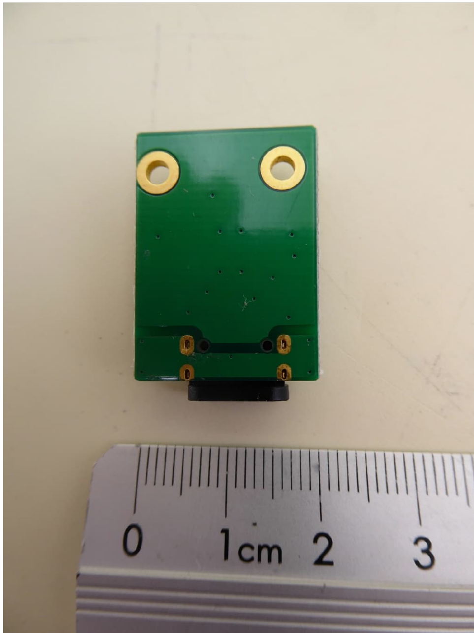
B650S / B650WS, USB PCB, bottom view
