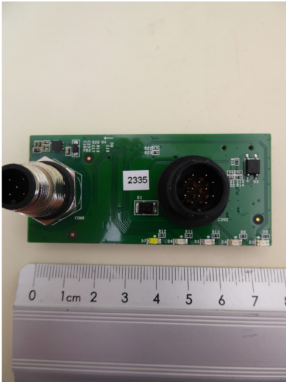
B650S / B650WS, connector PCB, top view
