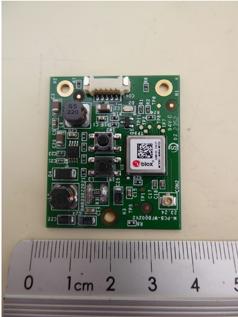
B650WS, Wi-Fi-module, top view
