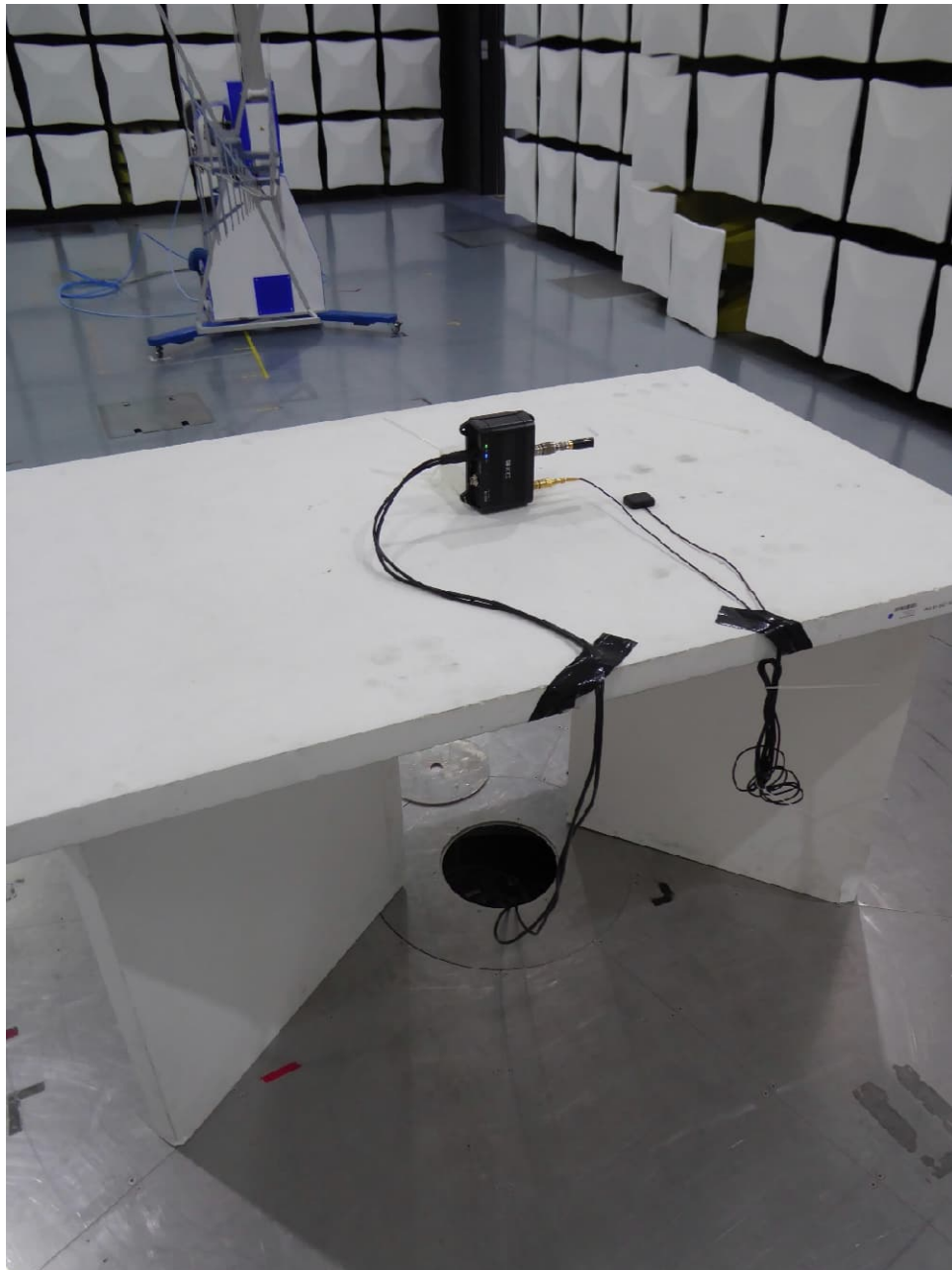
Test setup semi anechoic chamber (30 MHz to 1 GHz, position 2)
