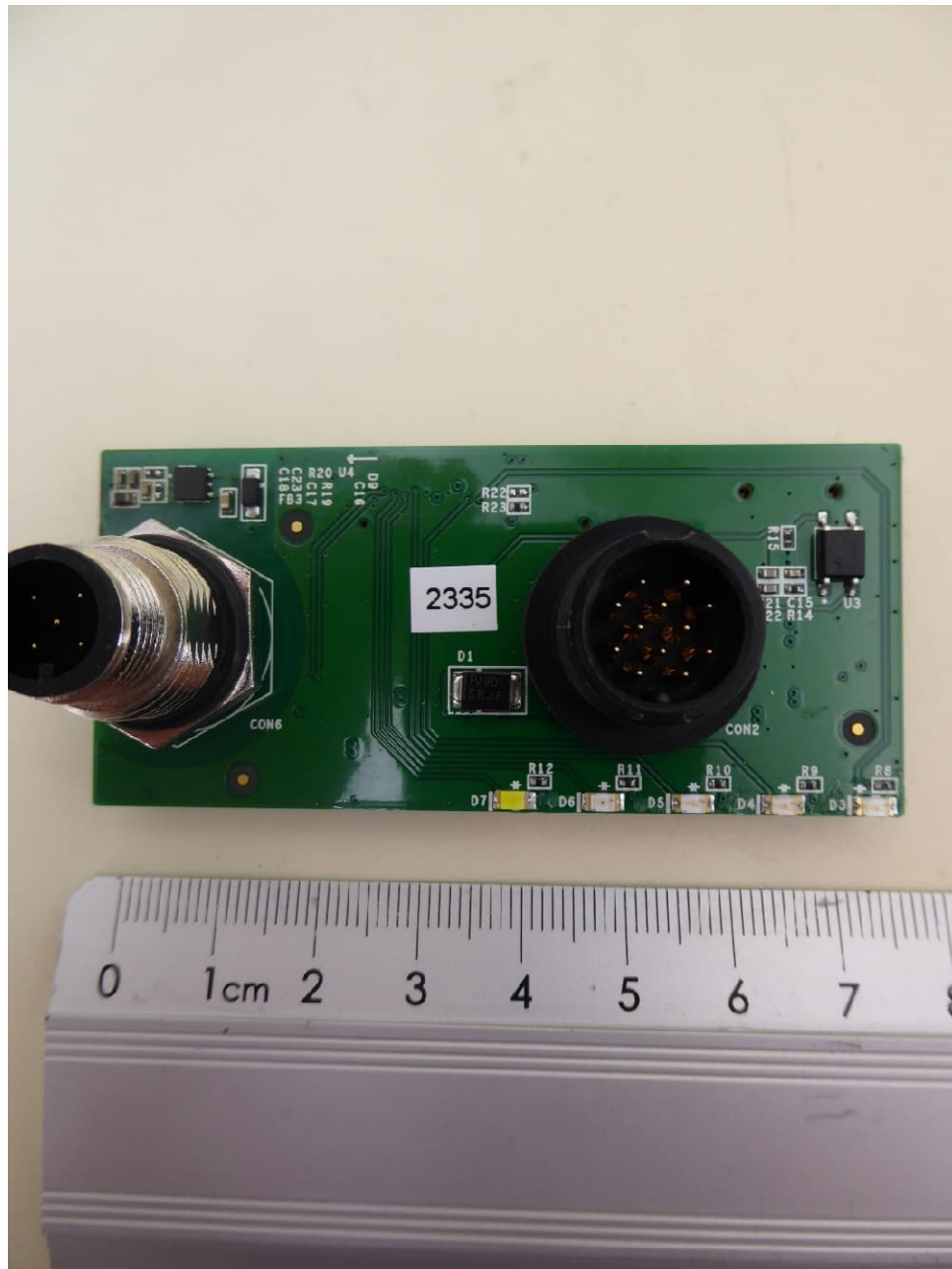
B650 / B650W, connector PCB, top view
