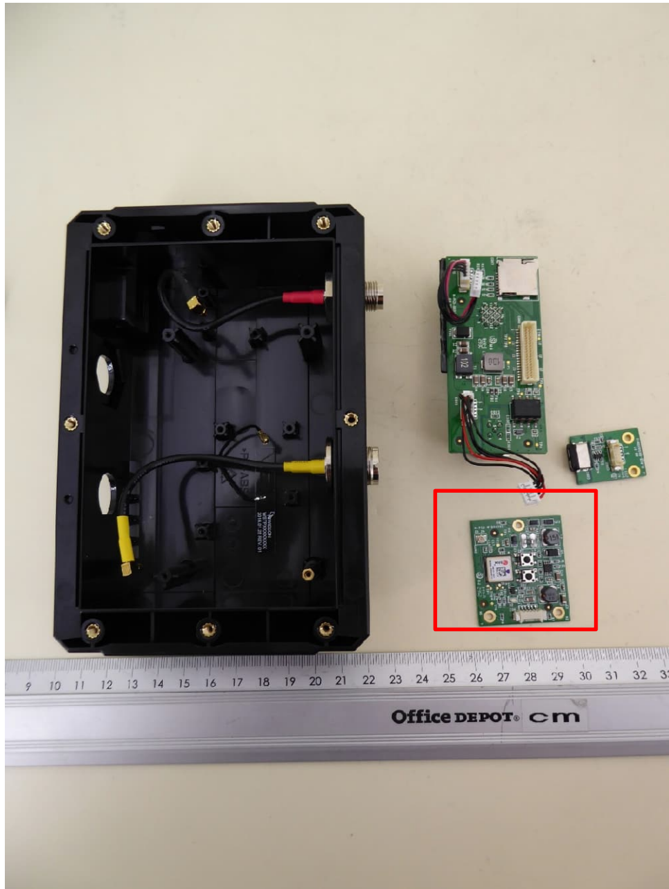
B650W (with certified Wifi Module FCC ID: WZ7-W151 / IC ID 9547A-W151), internal view 3, all PCBs removed
