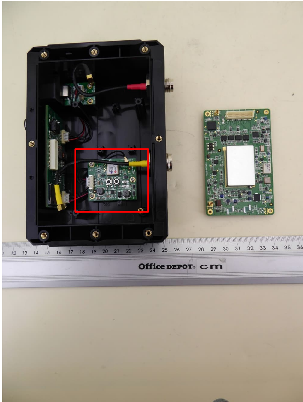
B650W, (with certified Wifi Module FCC ID: WZ7-W151 / IC ID 9547A-W151), internal view 2, main PCB removed
