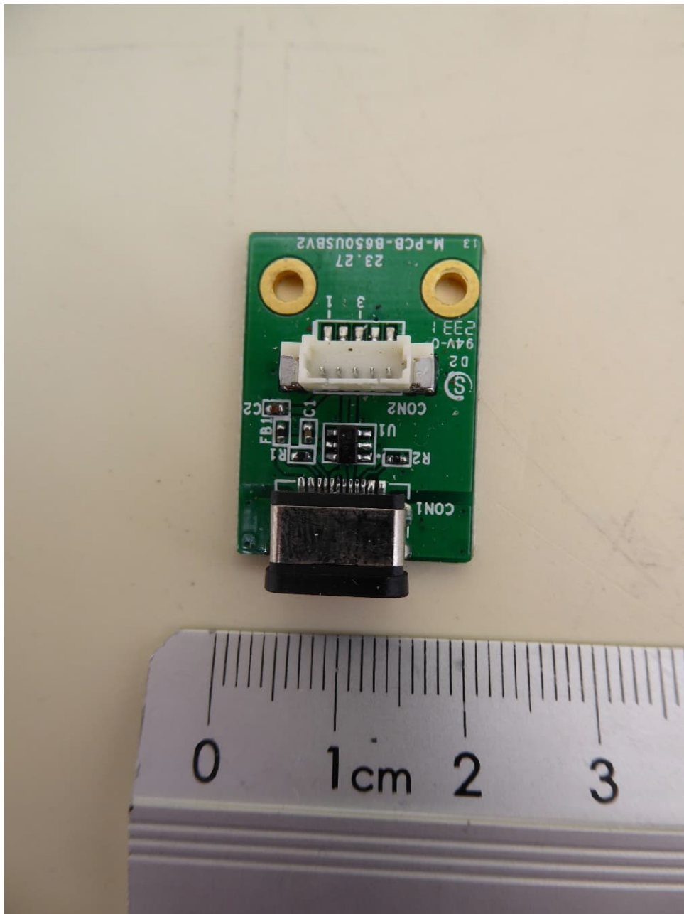
B650 / B650W, USB PCB, top view
