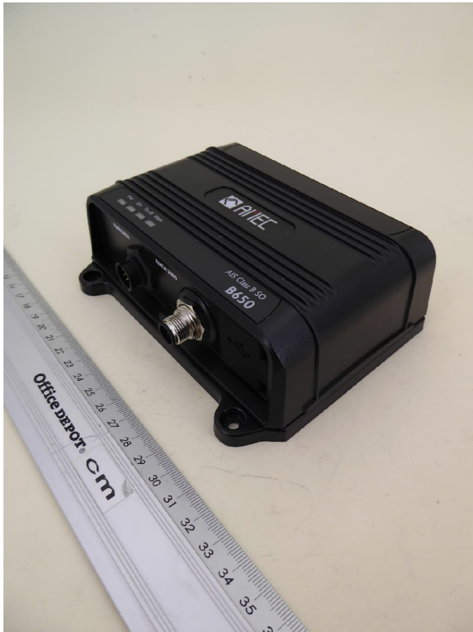
B650, 3-D-view 1
