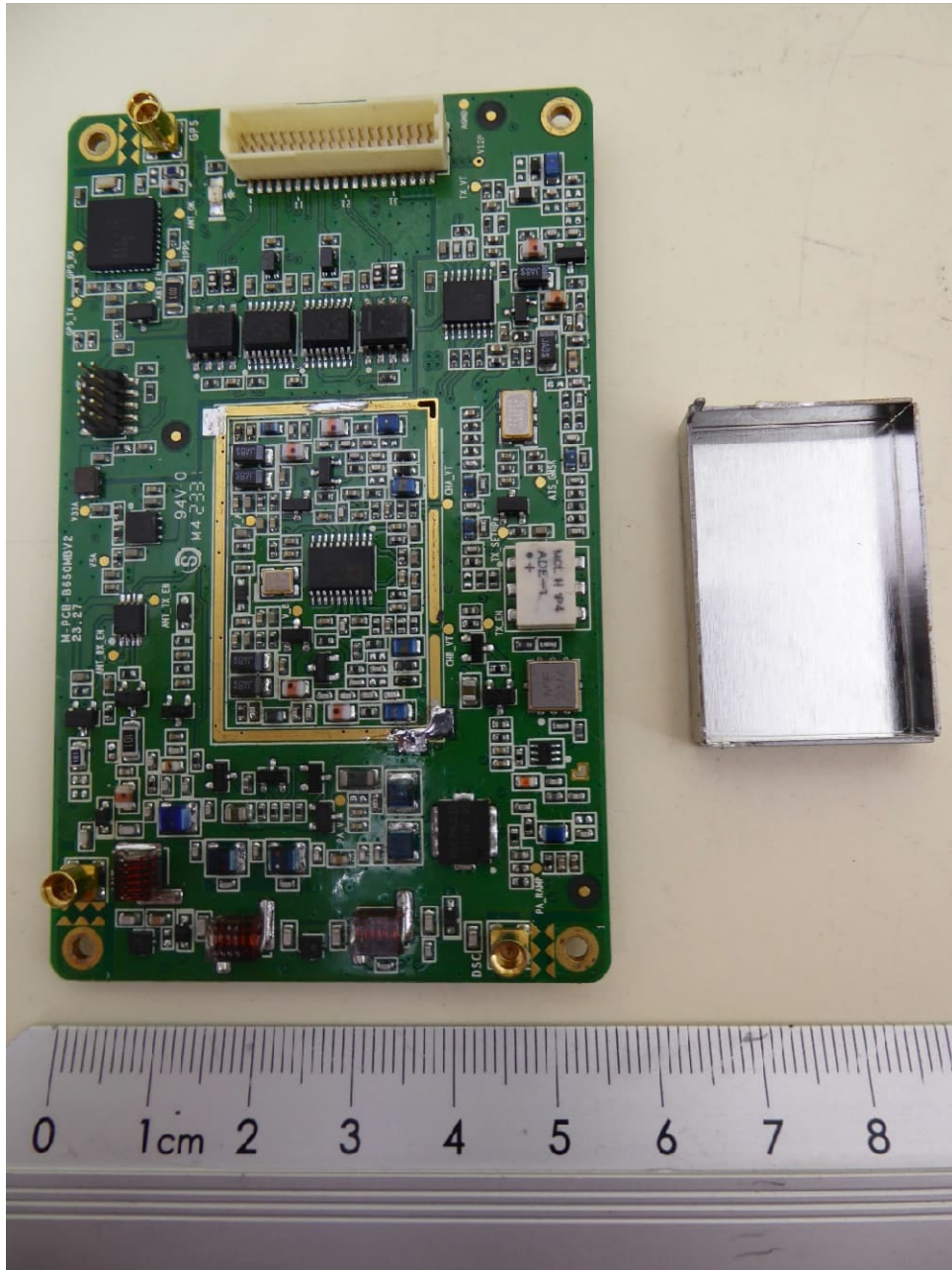
B620S / B620WS, main PCB, top view, shielding removed
