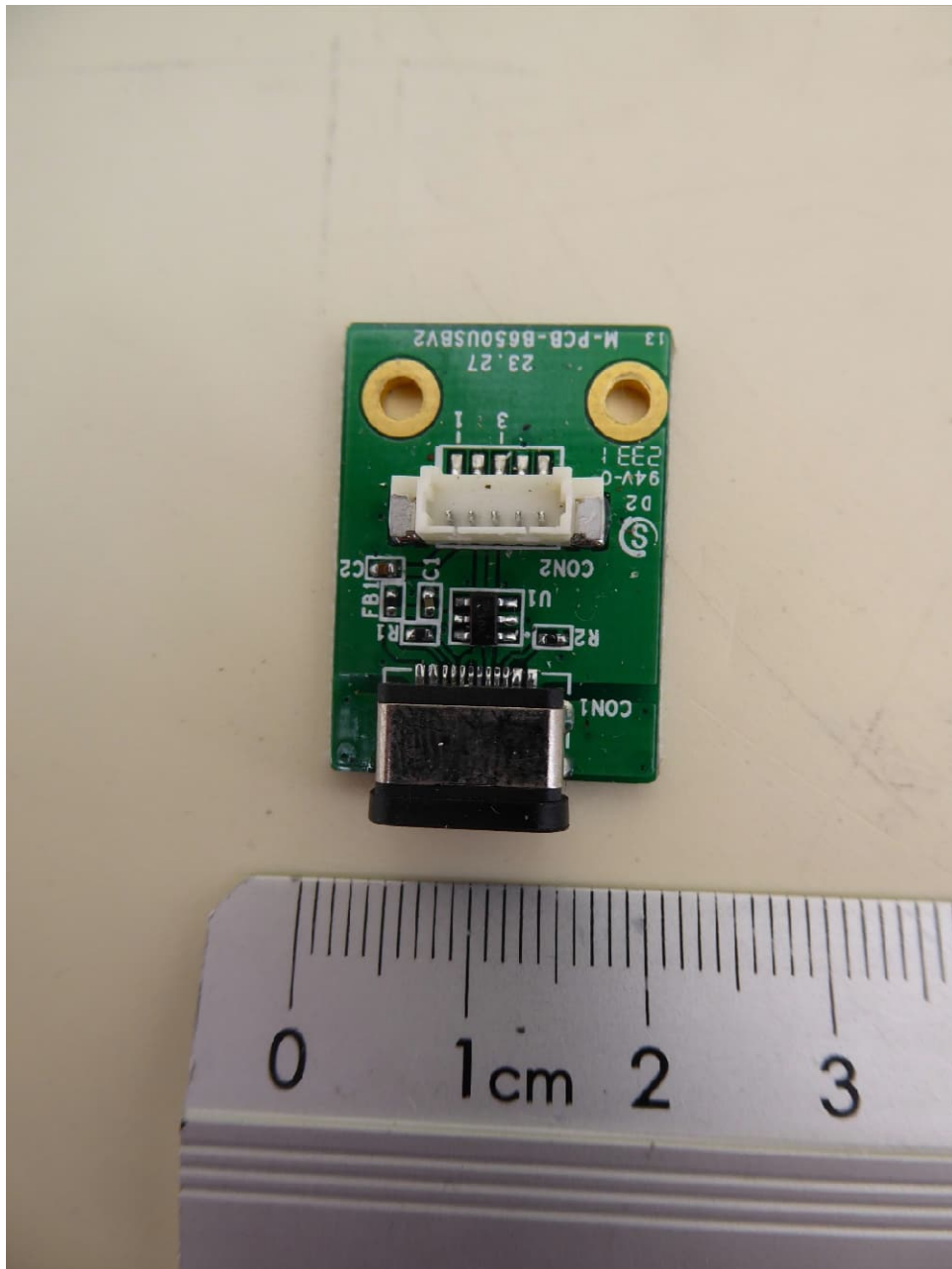
B620S / B620WS, USB PCB, top view
