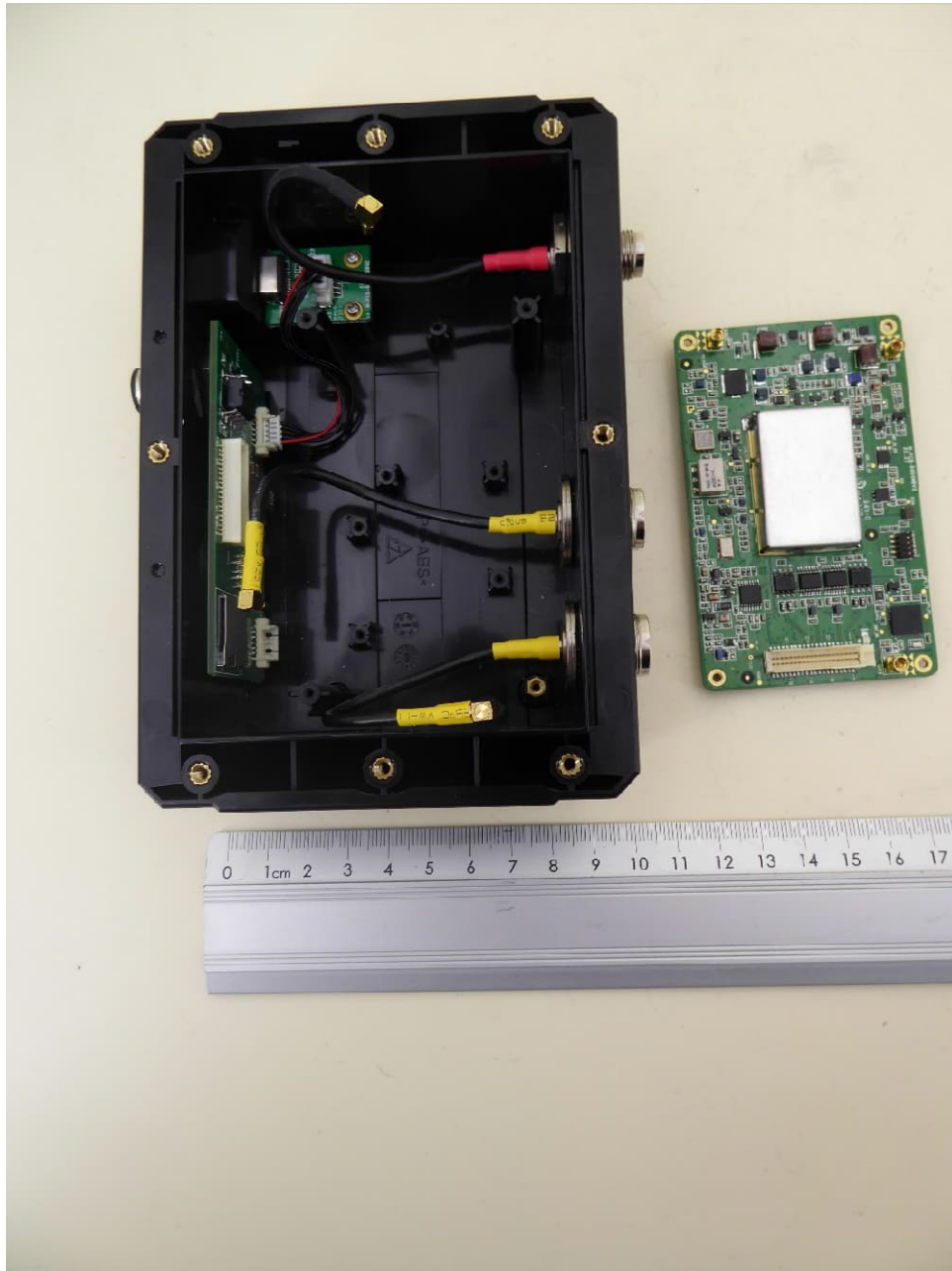
B620S, internal view 2, main PCB removed
