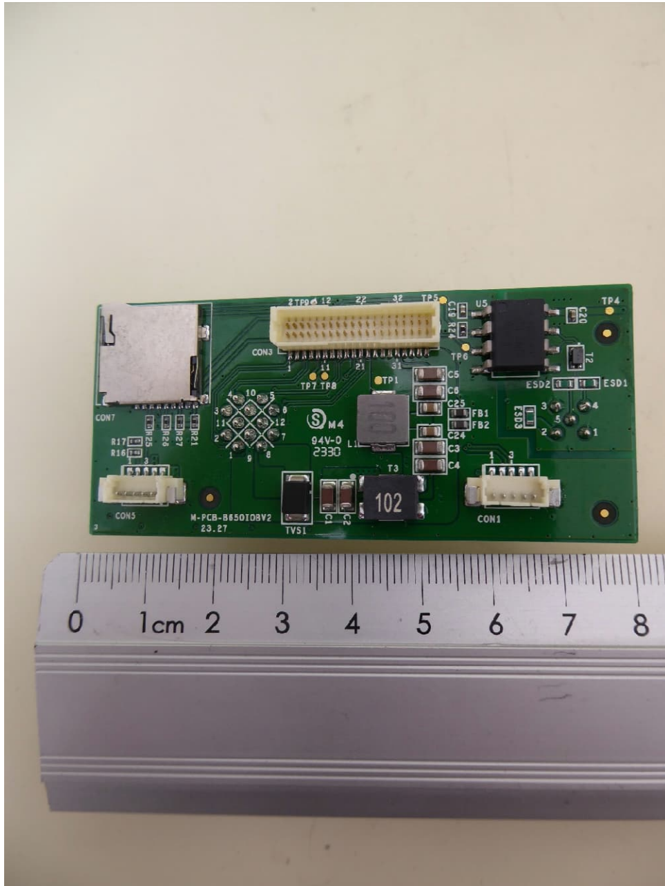
B620S / B620WS, connector PCB, bottom view
