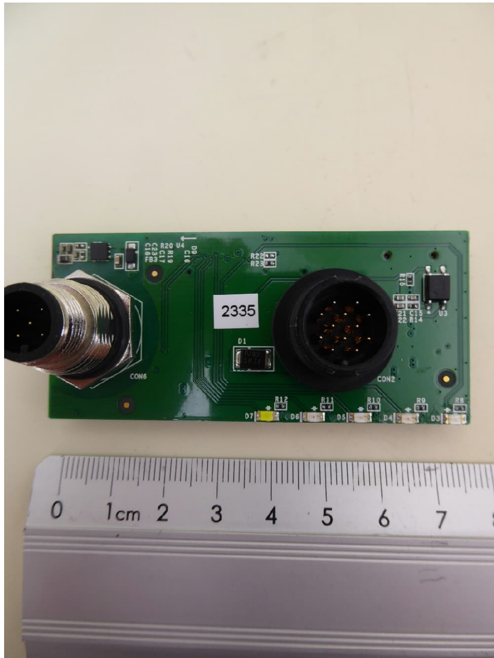
B620S / B620WS, connector PCB, top view
