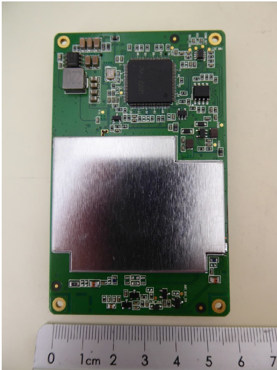
B620S / B620WS, main PCB, bottom view
