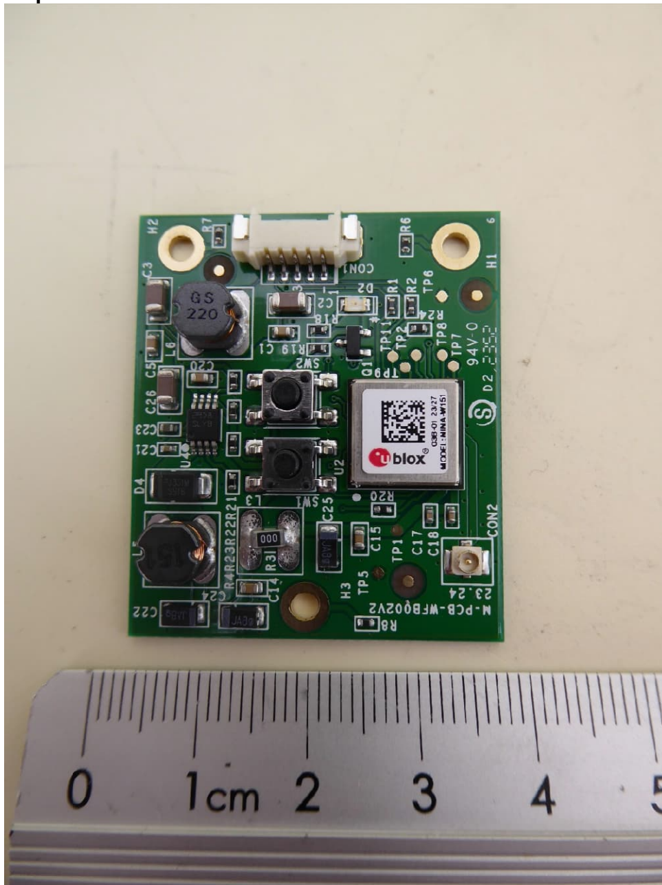
B620WS, Wi-Fi-module, top view
