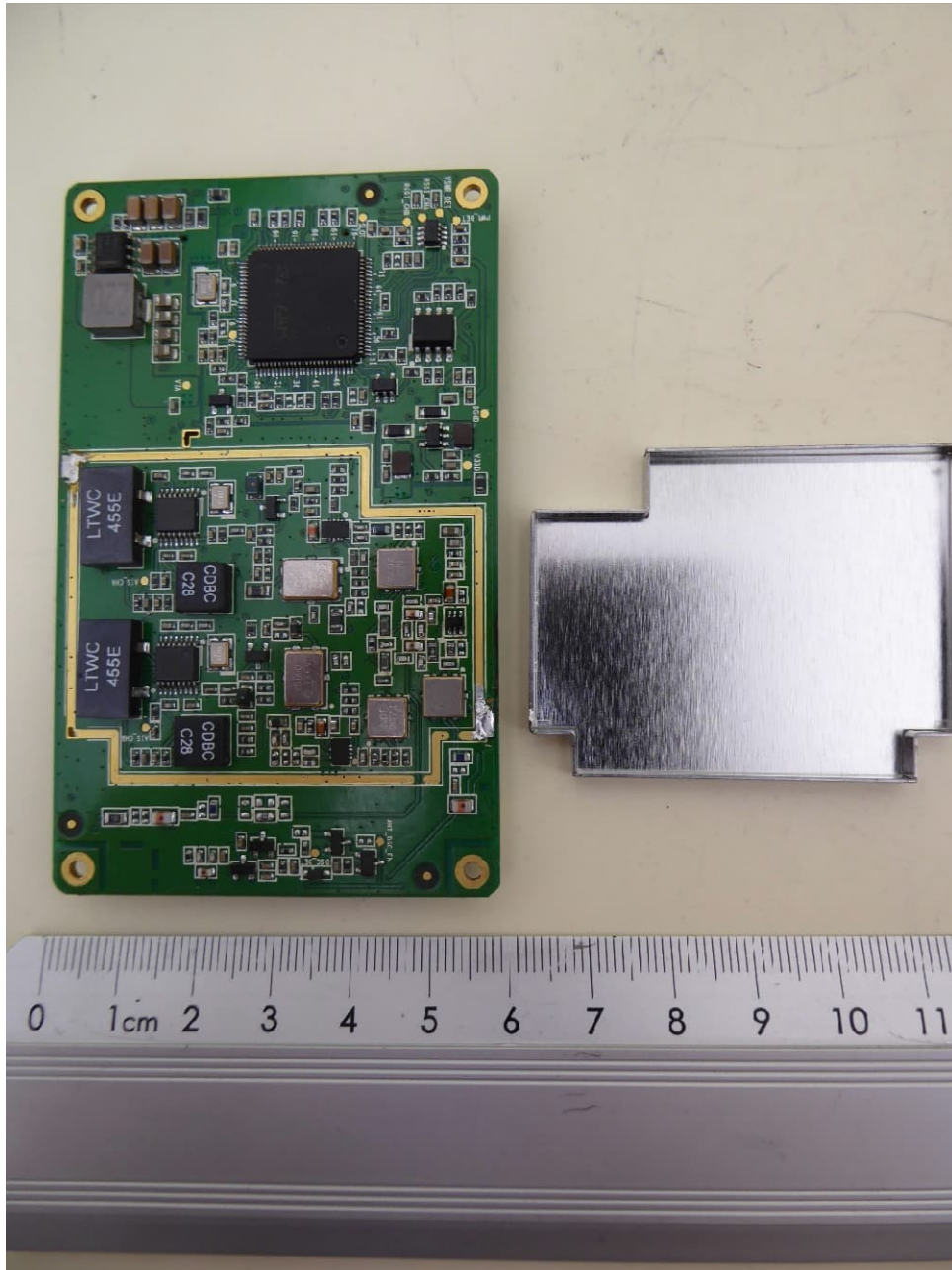
B620S / B620WS, main PCB, bottom view, shielding removed
