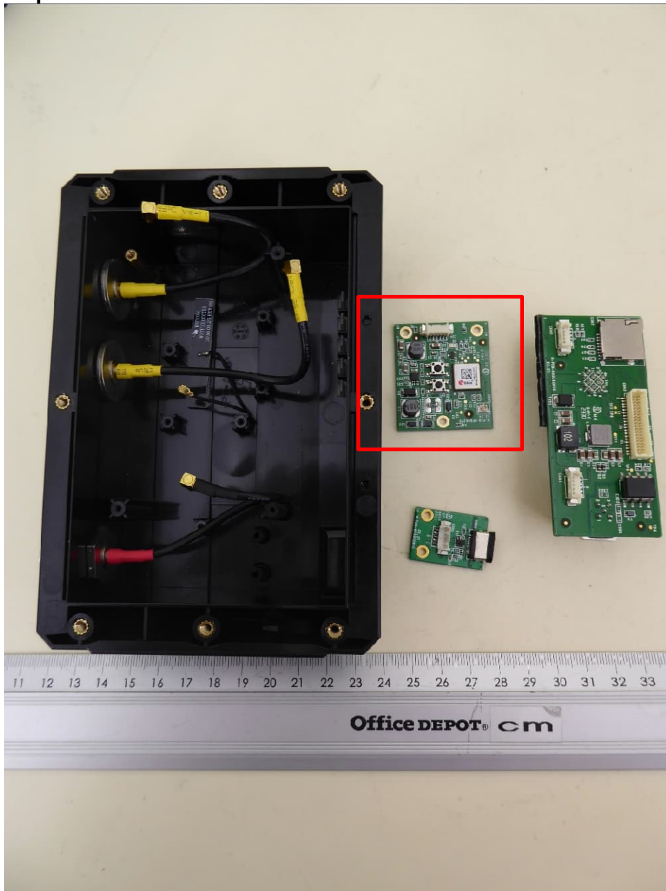
B620WS (with certified Wifi Module FCC ID: WZ7-W151 / IC ID 9547A-W151), internal view 3, all PCBs removed
