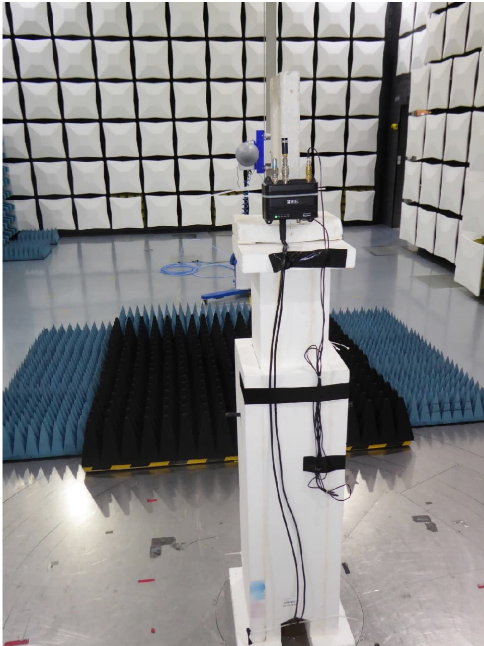
Test setup semi anechoic chamber (1 GHz to 2 GHz, position 3)
