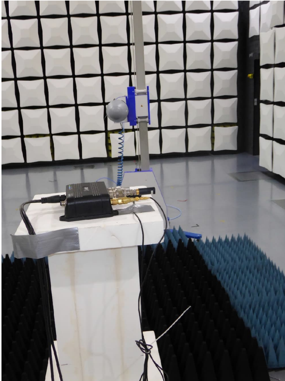
Test setup semi anechoic chamber (1 GHz to 2 GHz, position 1)
