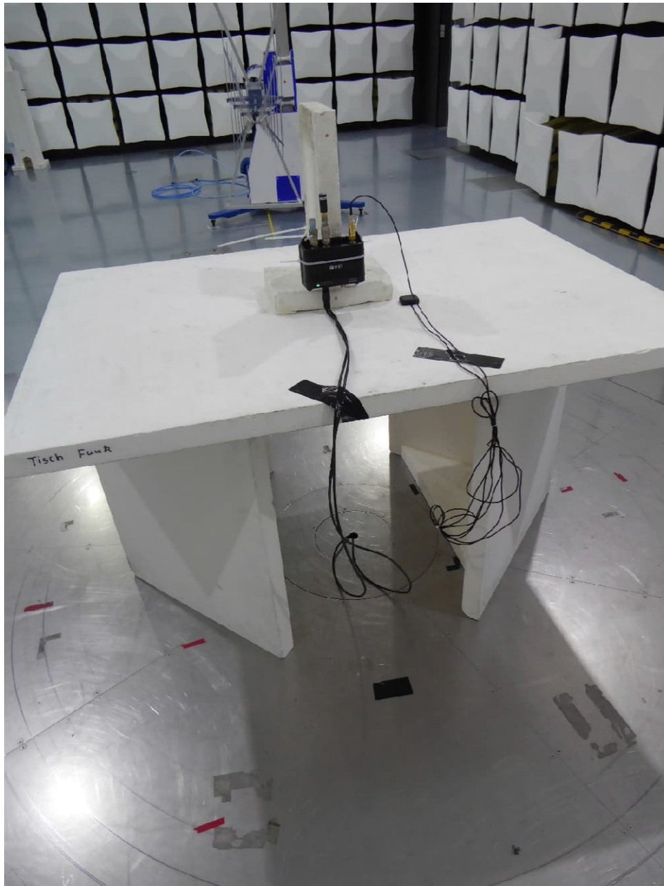
Test setup semi anechoic chamber (30 MHz to 1 GHz, position 3)
