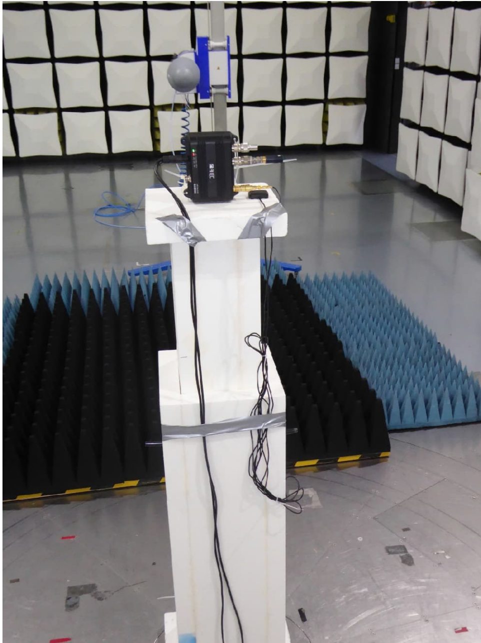
Test setup semi anechoic chamber (1 GHz to 2 GHz, position 2)
