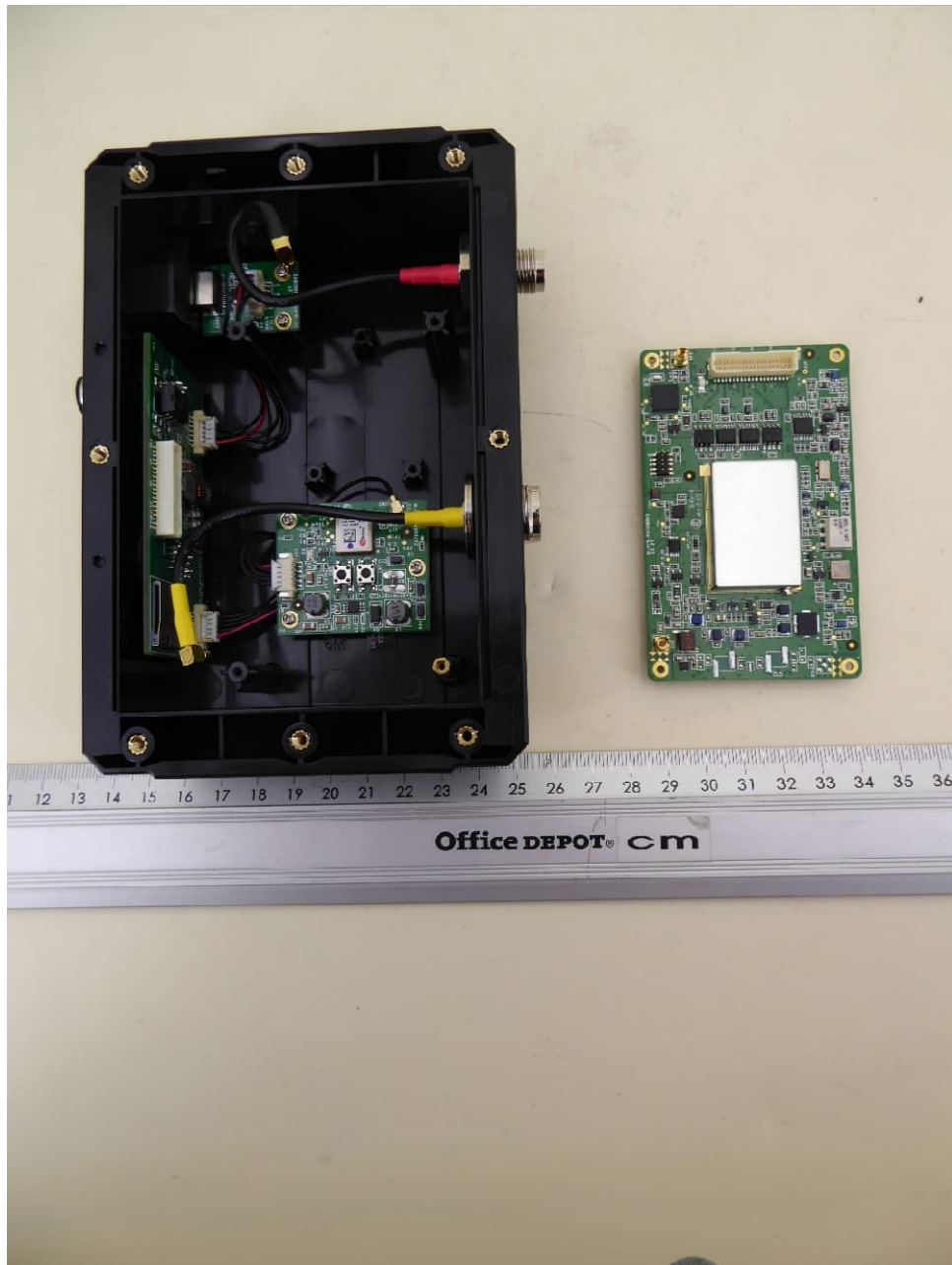
B620W, internal view 2, main PCB removed
