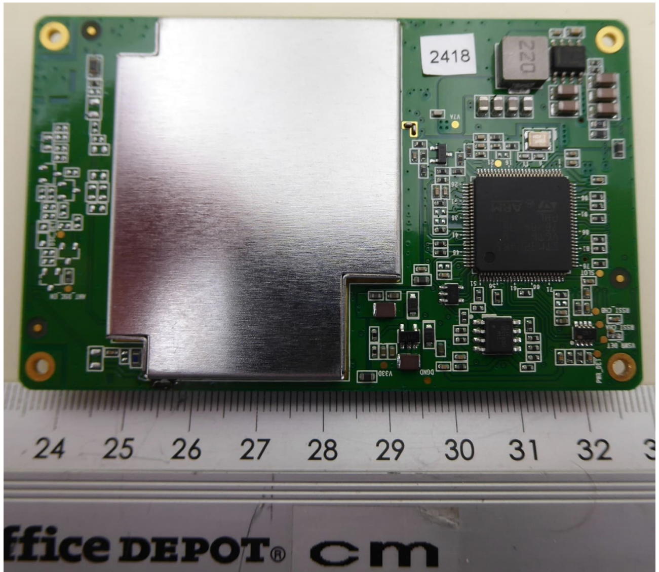
Main PCB – bottom view
