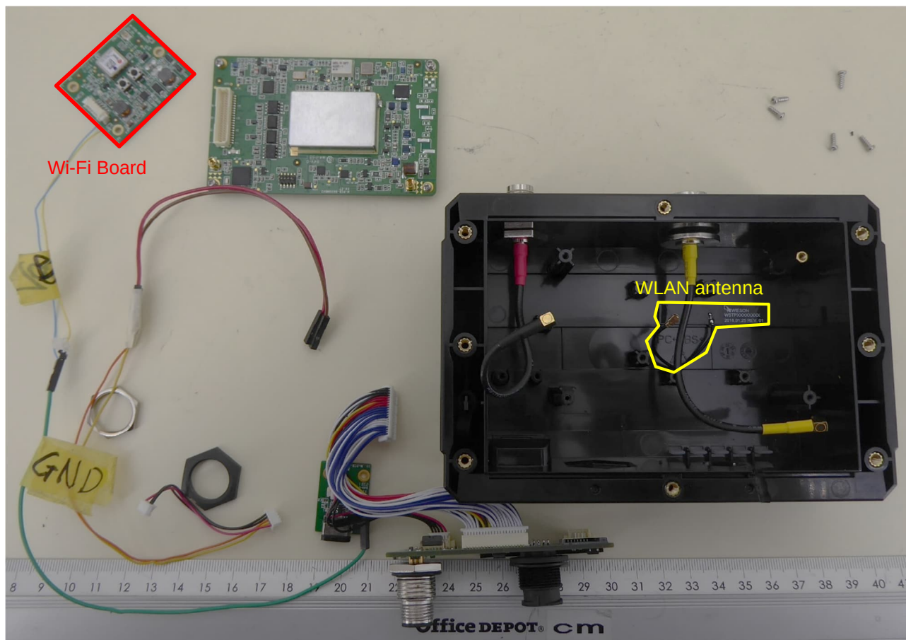
EUT disassembled
