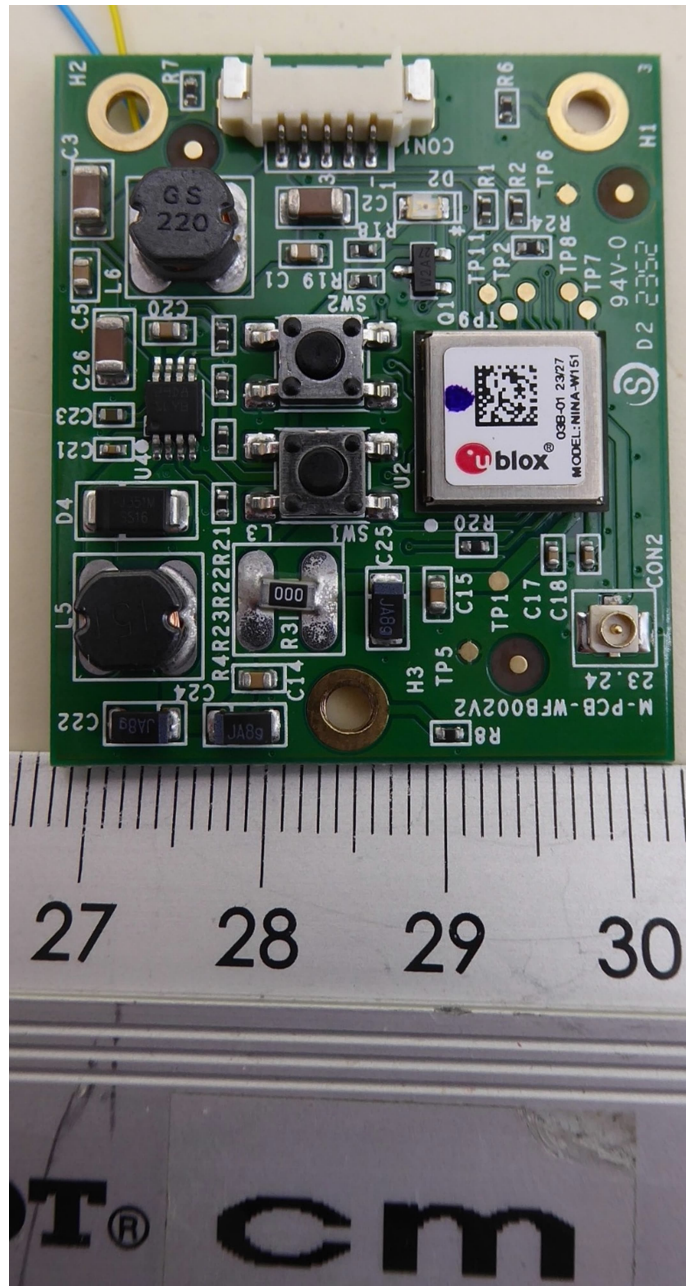
Wi-Fi Board – top view
