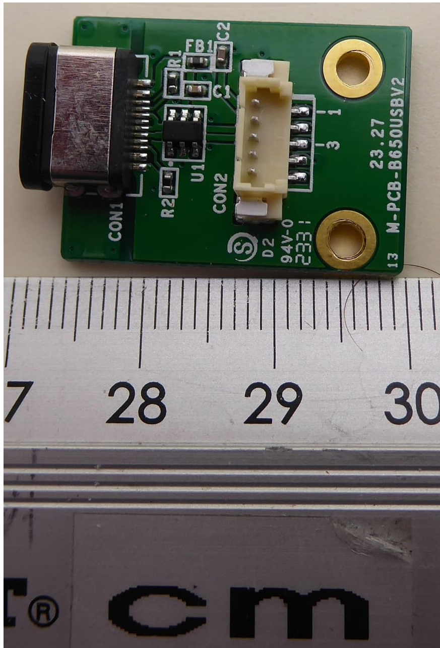
USB PCB– top view
