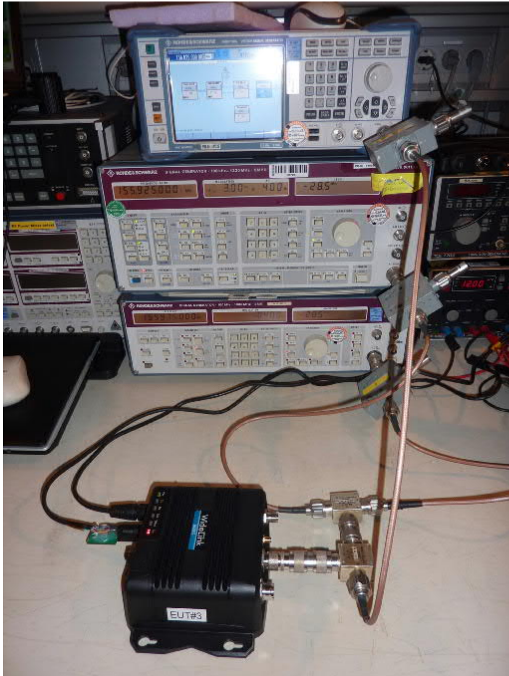
190014_c.jpg: WIDELINK B600S, test setup shielded chamber
