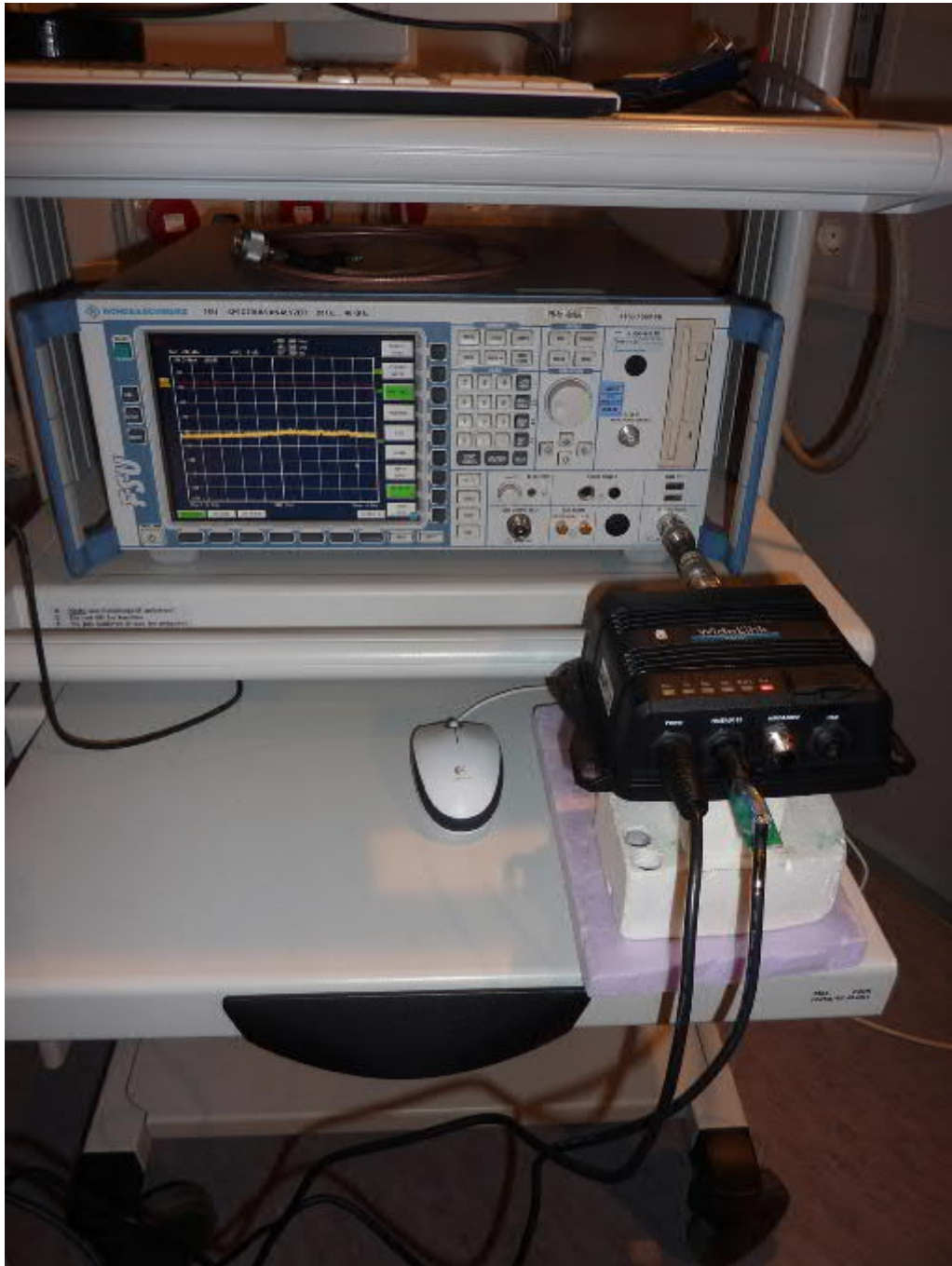
190014_b.jpg: WIDELINK B600S, test setup shielded chamber
