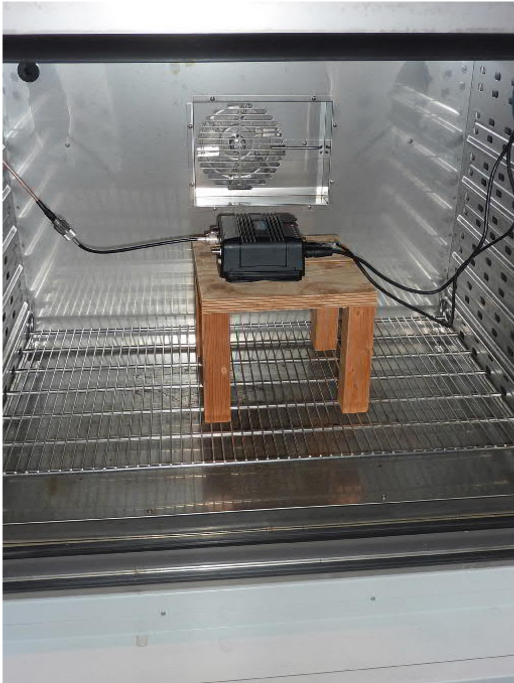
190014_e.jpg: WIDELINK B600S, test setup temperature chamber
