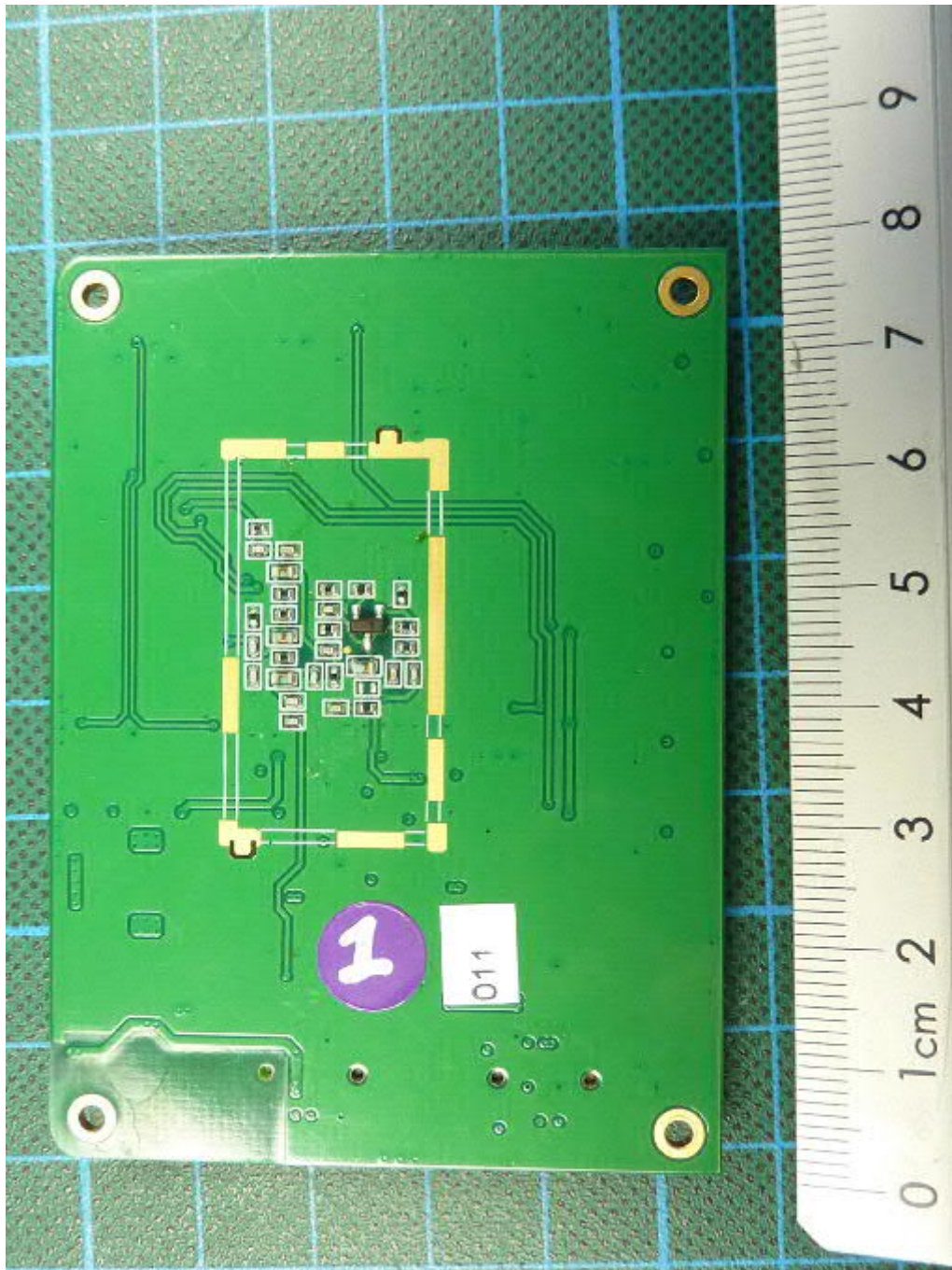
190014_14.jpg: WIDELINK B600S, PCB 1, bottom view
