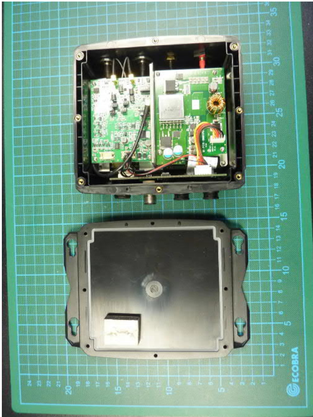
190014_6.jpg: WIDELINK B600S, internal view 1
