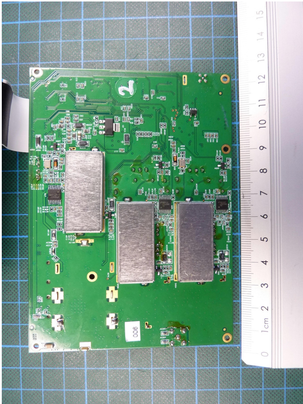
190014_10.jpg: WIDELINK B600S, PCB 3, bottom view
