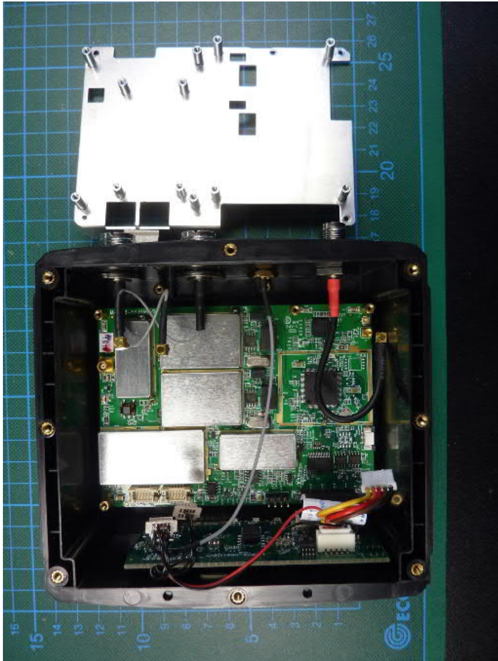
190014_8.jpg: WIDELINK B600S, internal view 3 (shielding removed)
