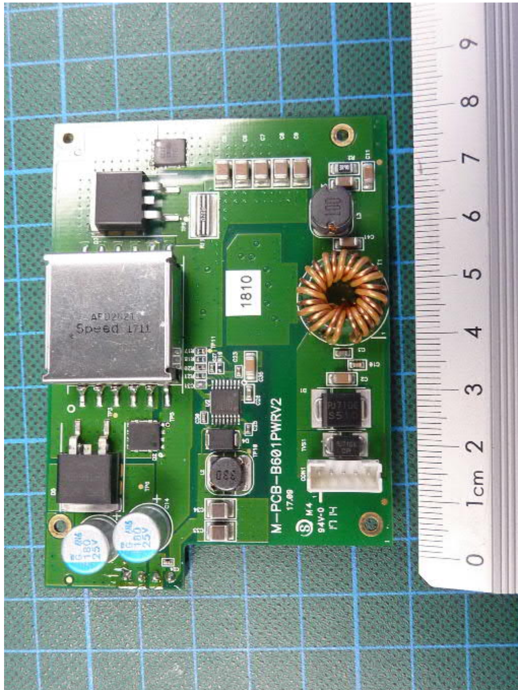
190014_15.jpg: WIDELINK B600S, PCB 2, top view
