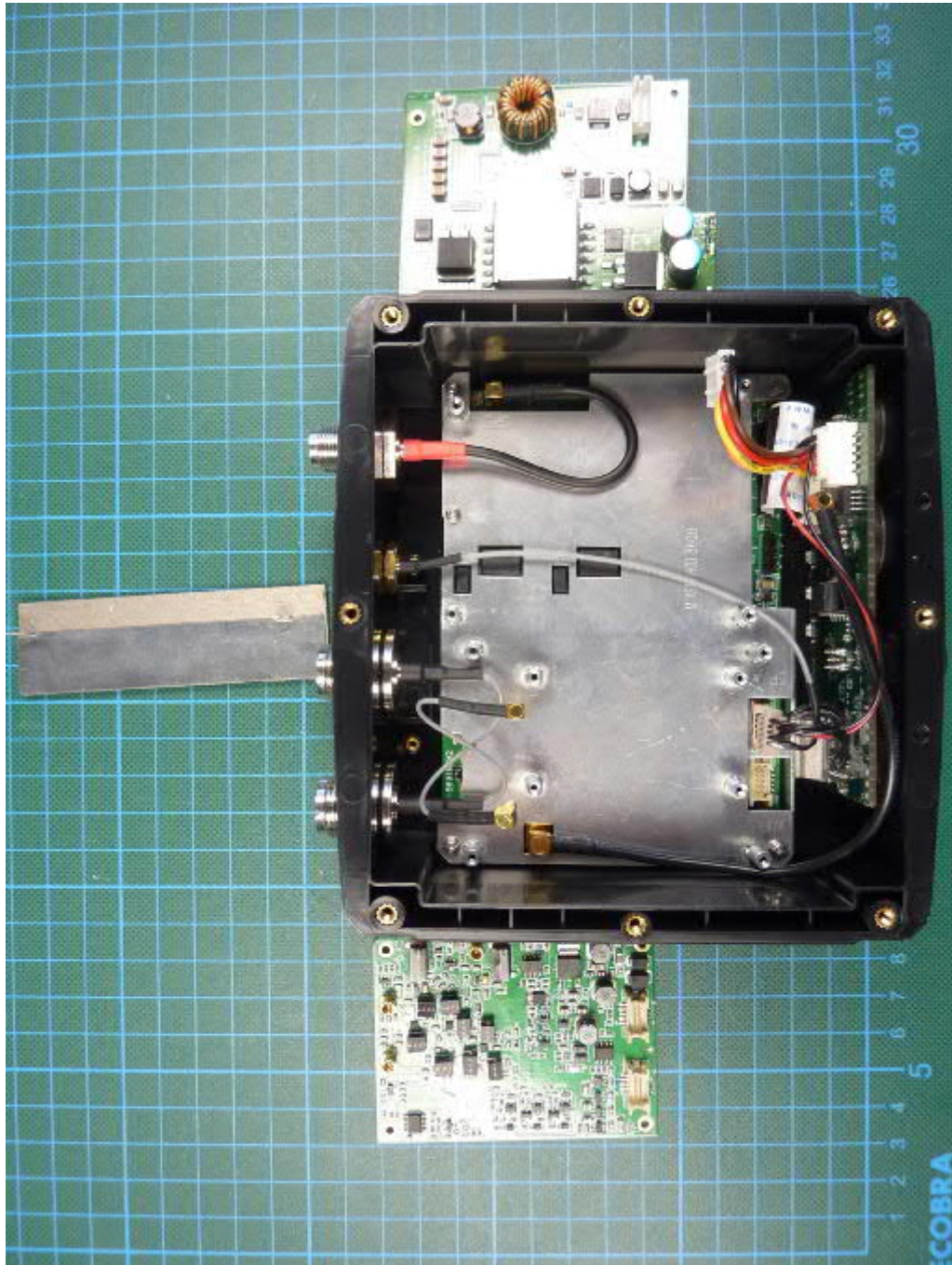
190014_7.jpg: WIDELINK B600S, internal view 2 (PCB 1 + 2 removed)
