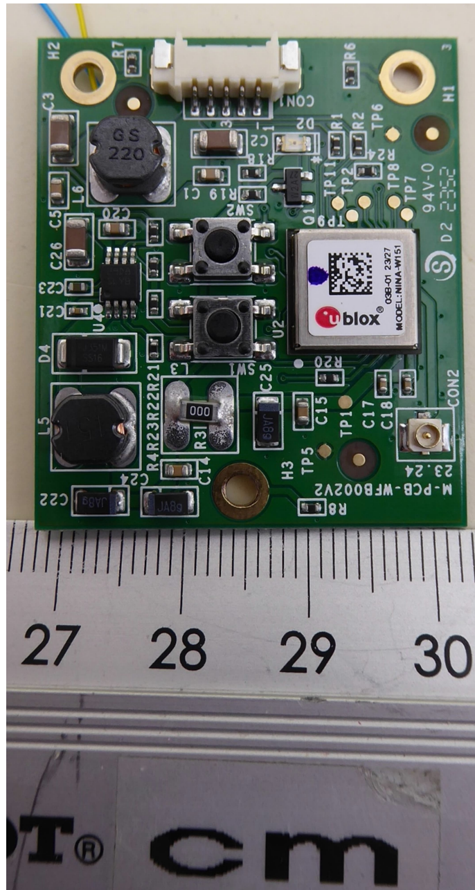
EUT – top view
